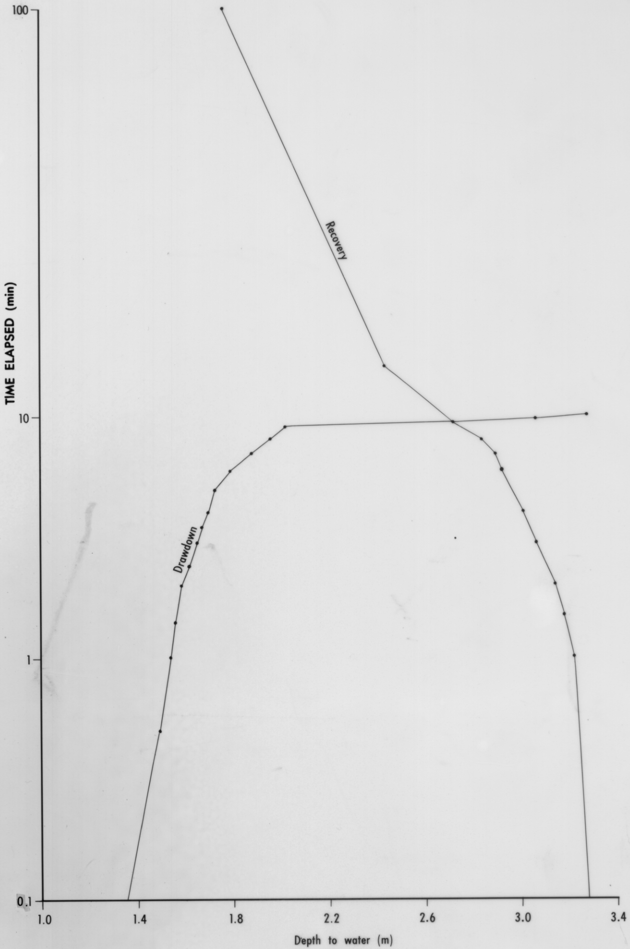
U/R 1977/37 FIG. 13 WANSTEAD FARM HOLE 5 DRAWDOWN AND RECOVERY
