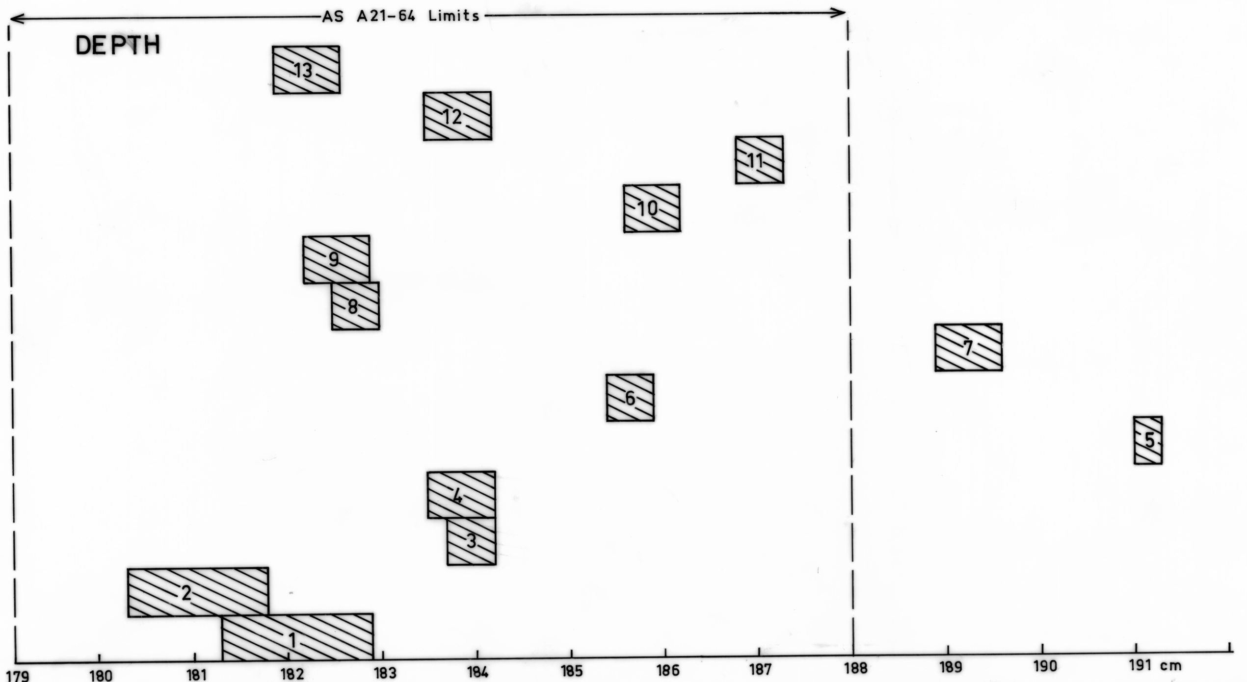
COMPARISON OF BRICK DIMENSIONS WITH SPECIFICATION REQUIREMENTS R767 (DEC 1977)
