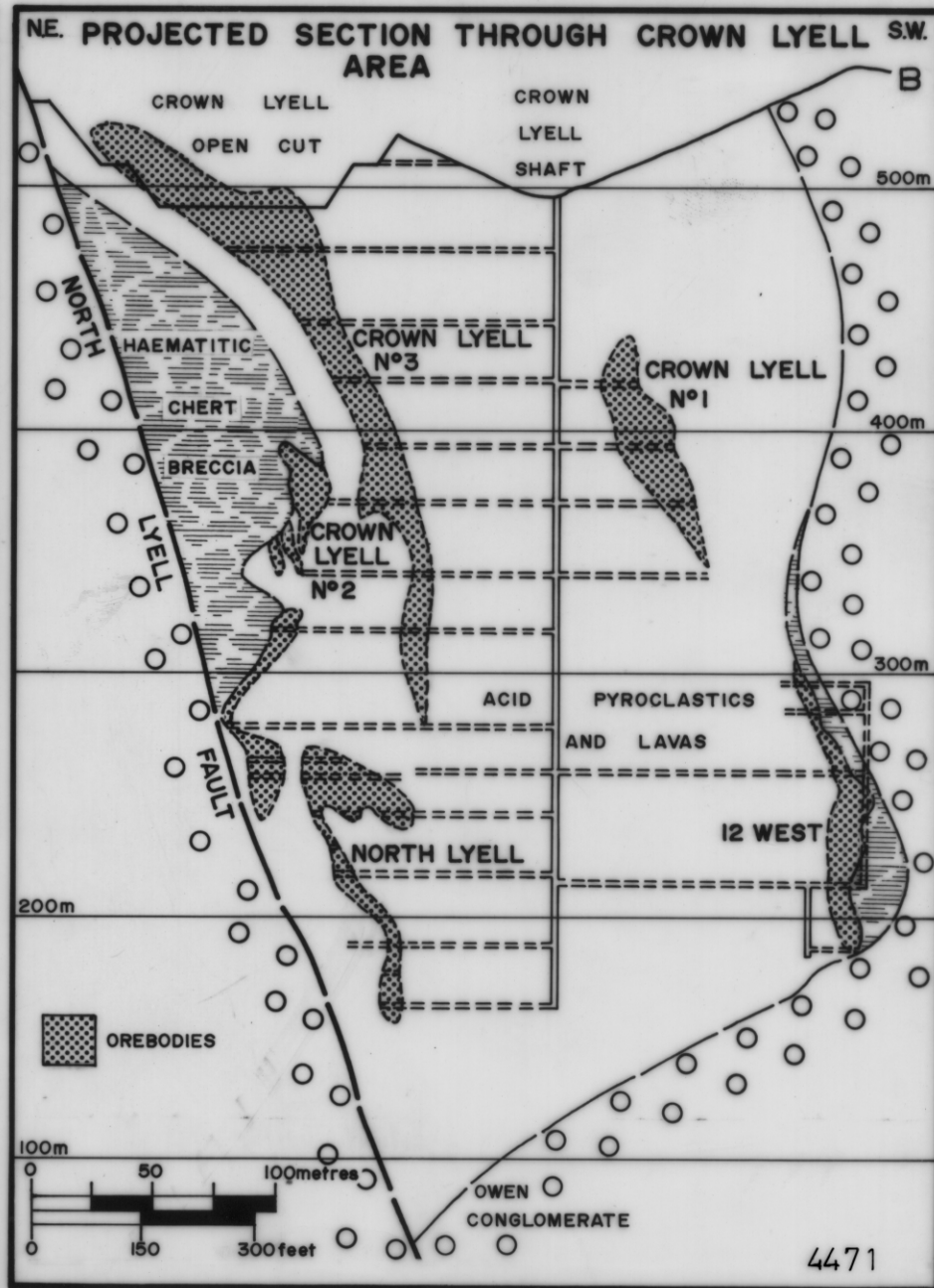
Section looking southeast through the Crown Lyell area
