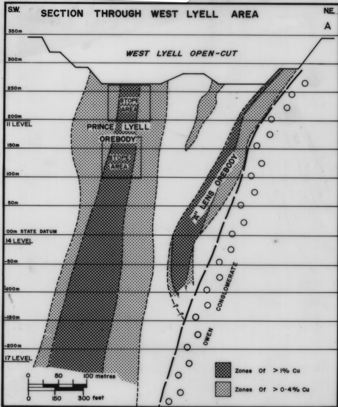
Section looking north-west through Prince Lyell orebody
