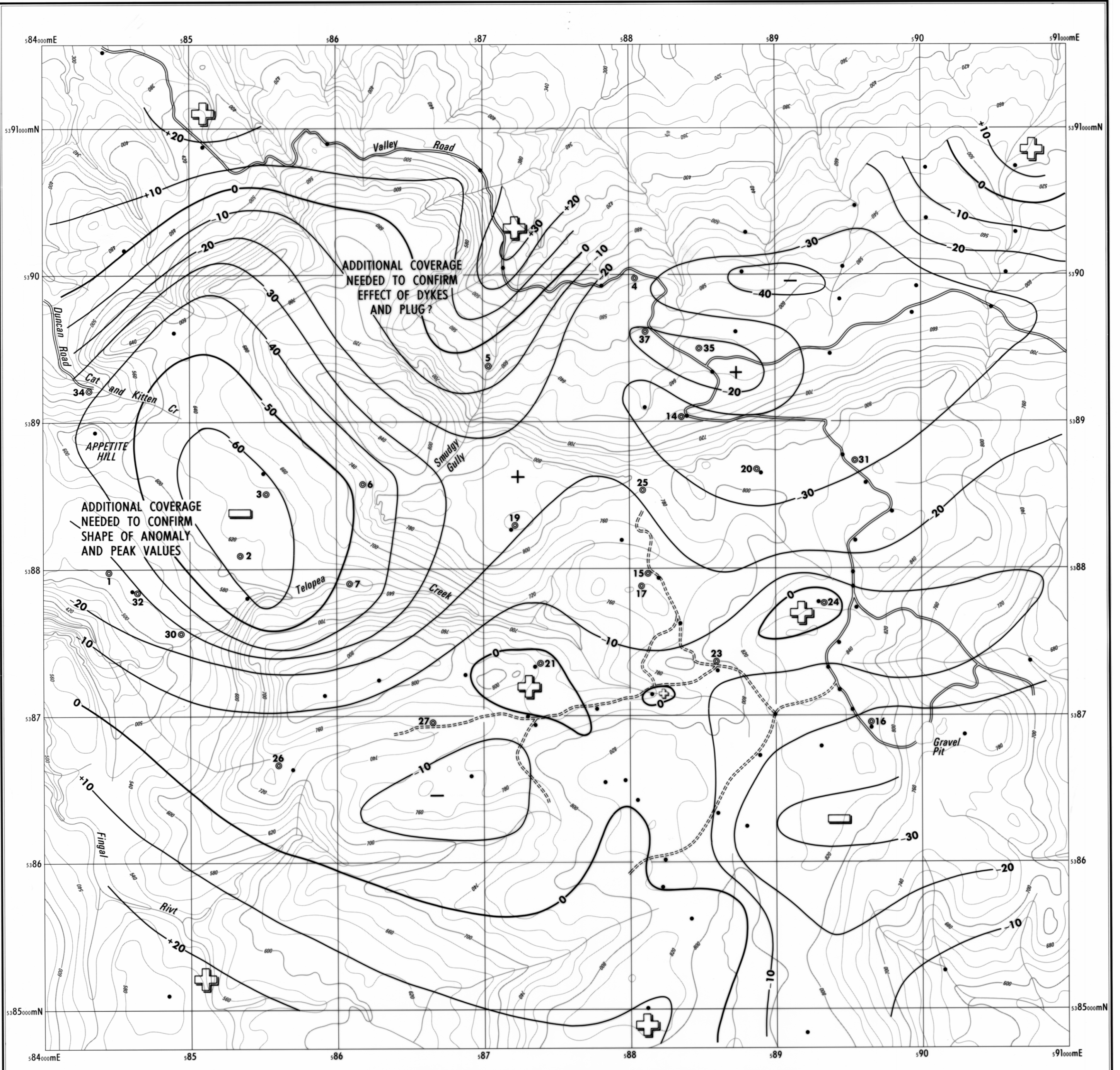
DETAIL OF RESIDUAL BOUGUER ANOMALIES SOUTH EAST OF THE DUNCAN MINE AND AROUND THE VALLEY GRID
