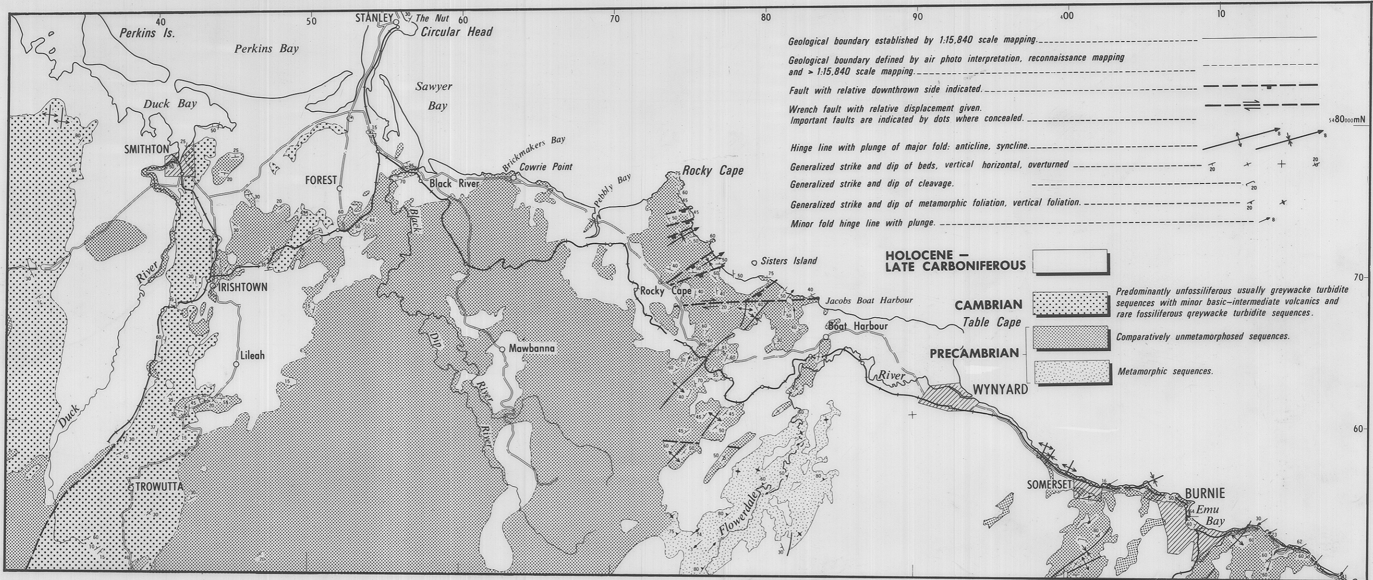
BASEMENT GEOLOGY, SMITHTON - BURNIE
