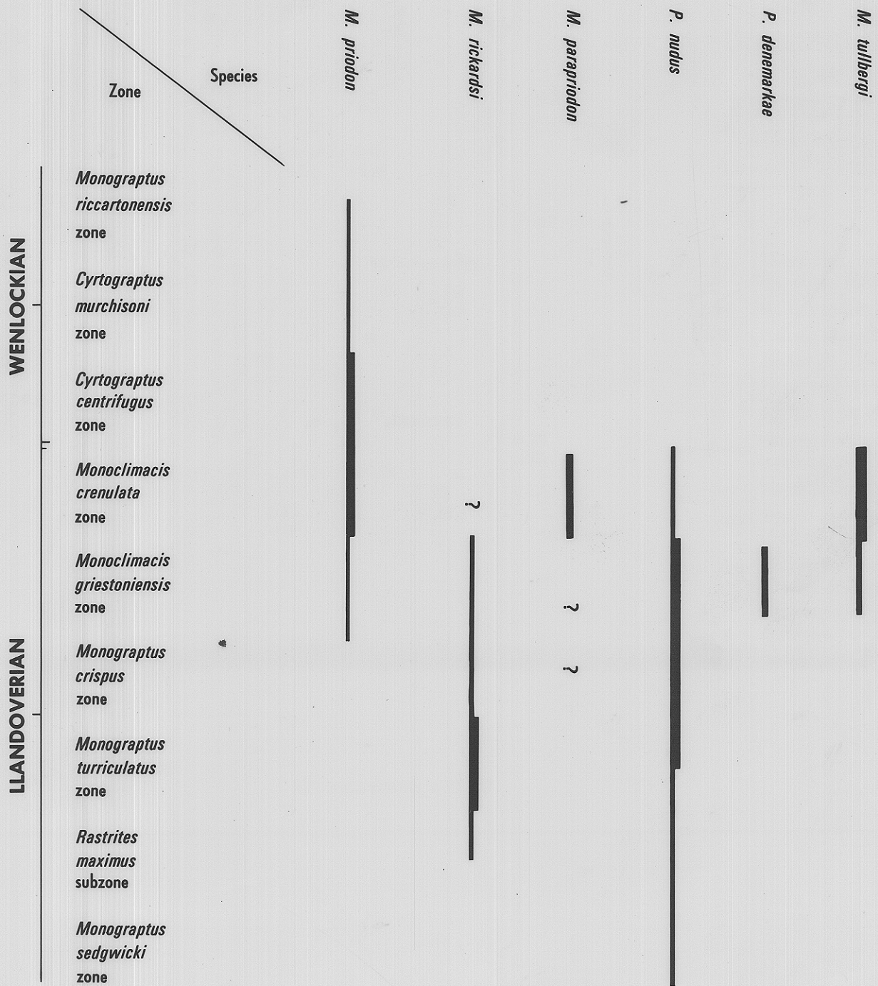
RANGES OF GRAPTOLITES [after RICKARDS (1976)]
