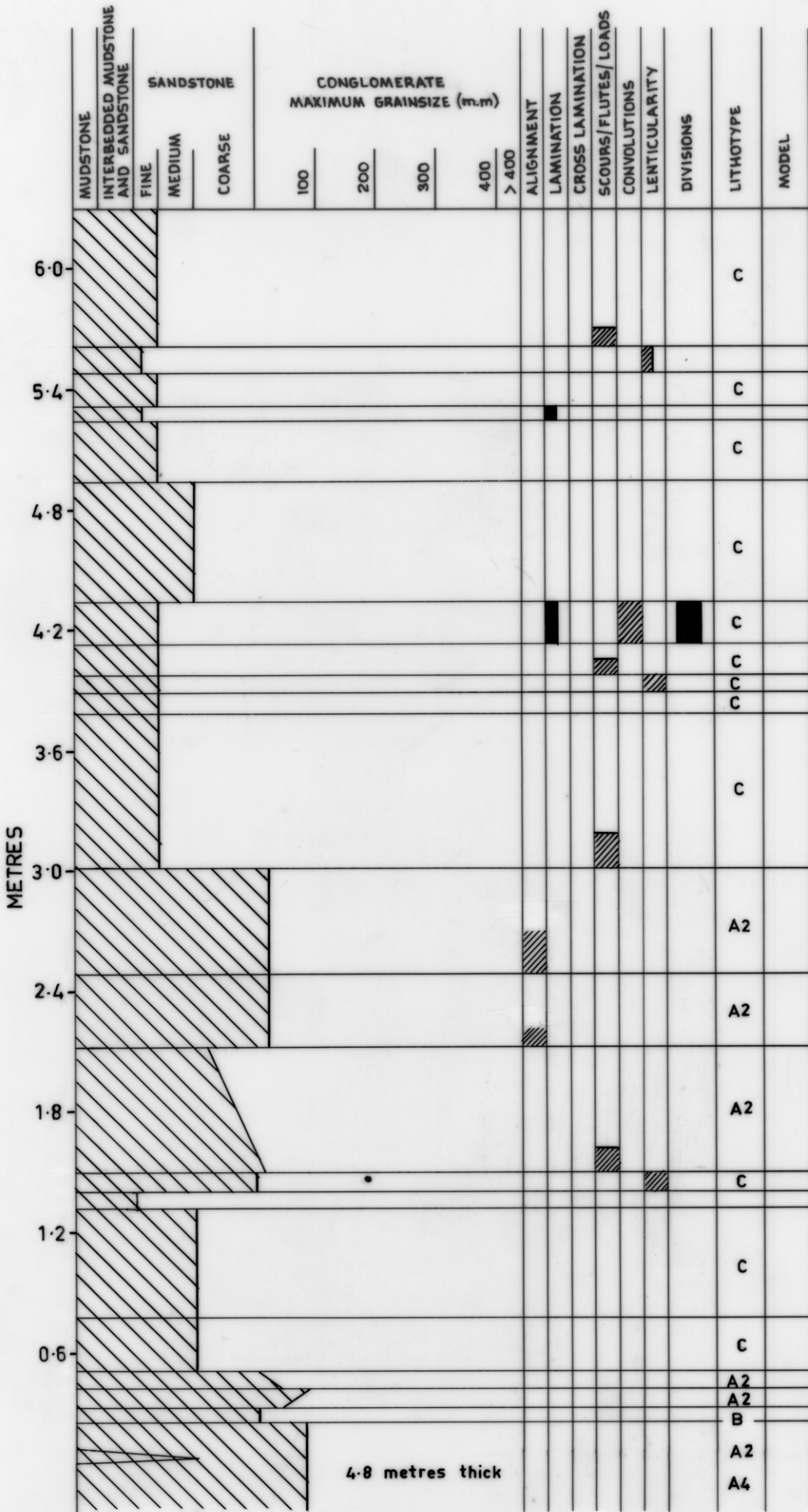
STRATIGRAPHIC SEQUENCE , BASE OF JOAN POINT SANDSTONE
