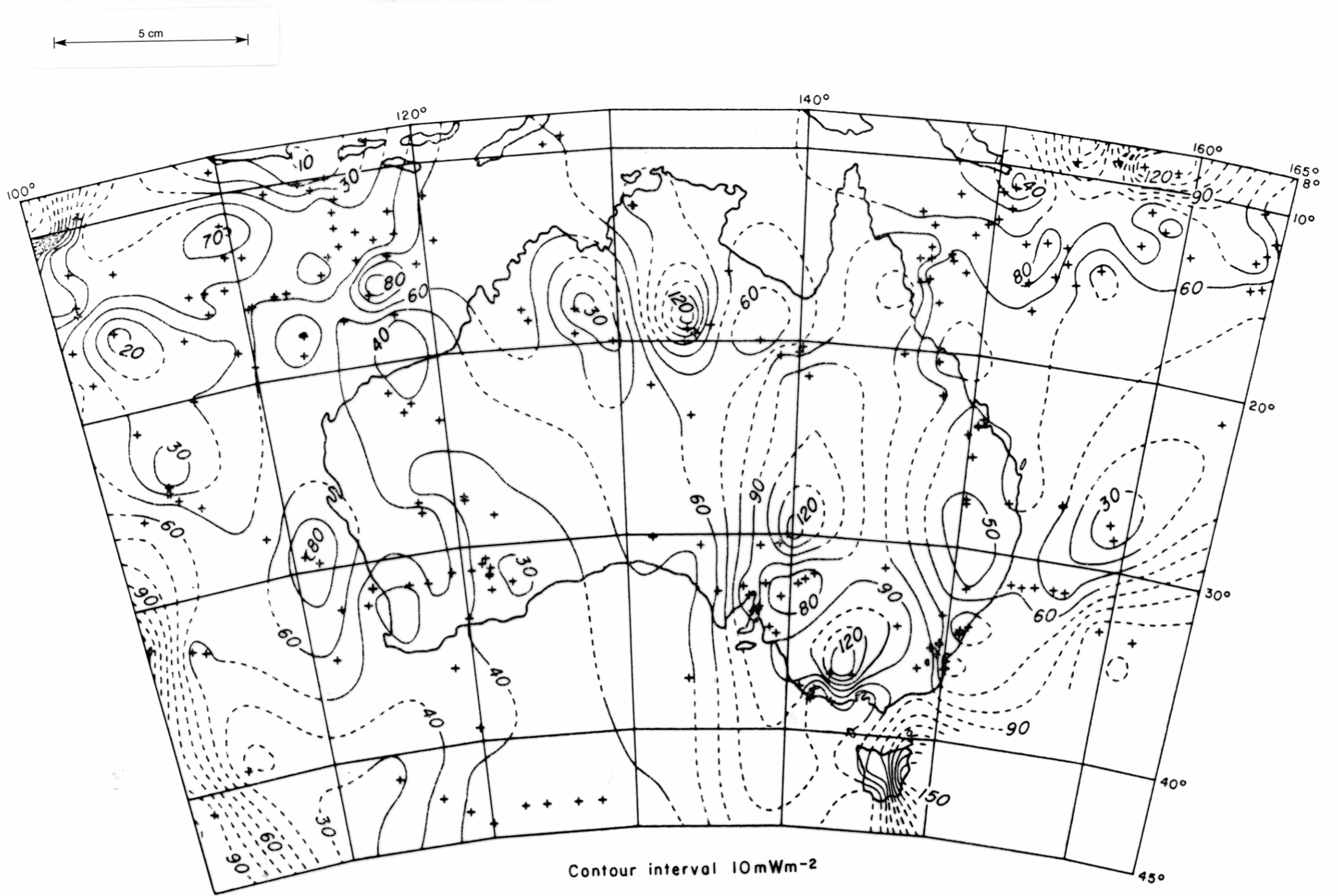
Heat-flow for the Australian region. Contours derived from a 1° grid of values.
