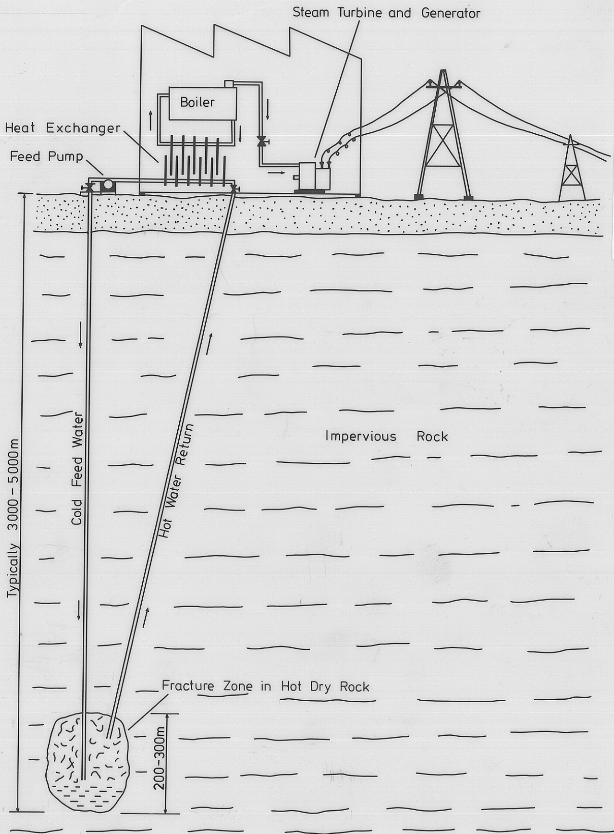
HOT DRY ROCK POWER STATION
