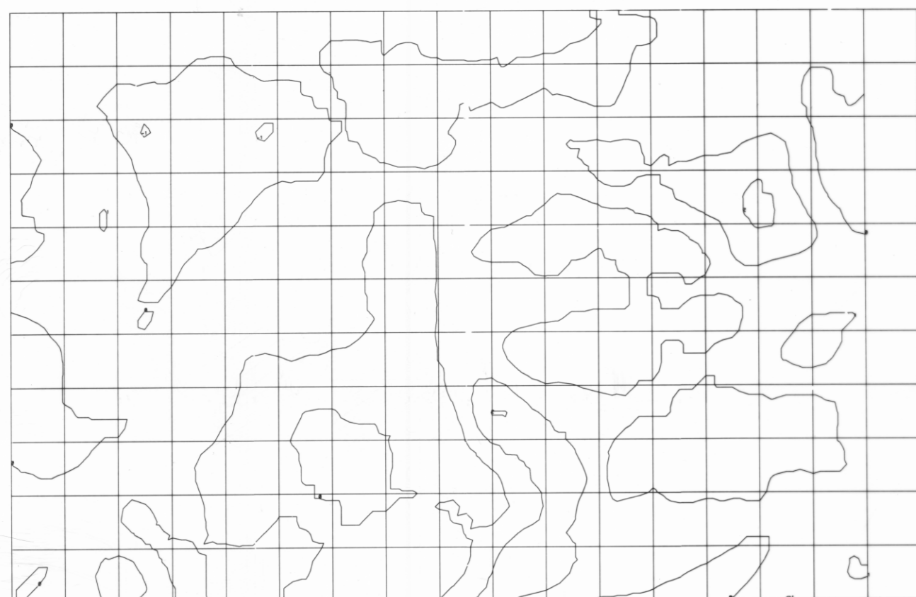
Fig. 28 CONTINUATION RESIDUALS AT 0.85 km. FINGAL TIER SURVEY
