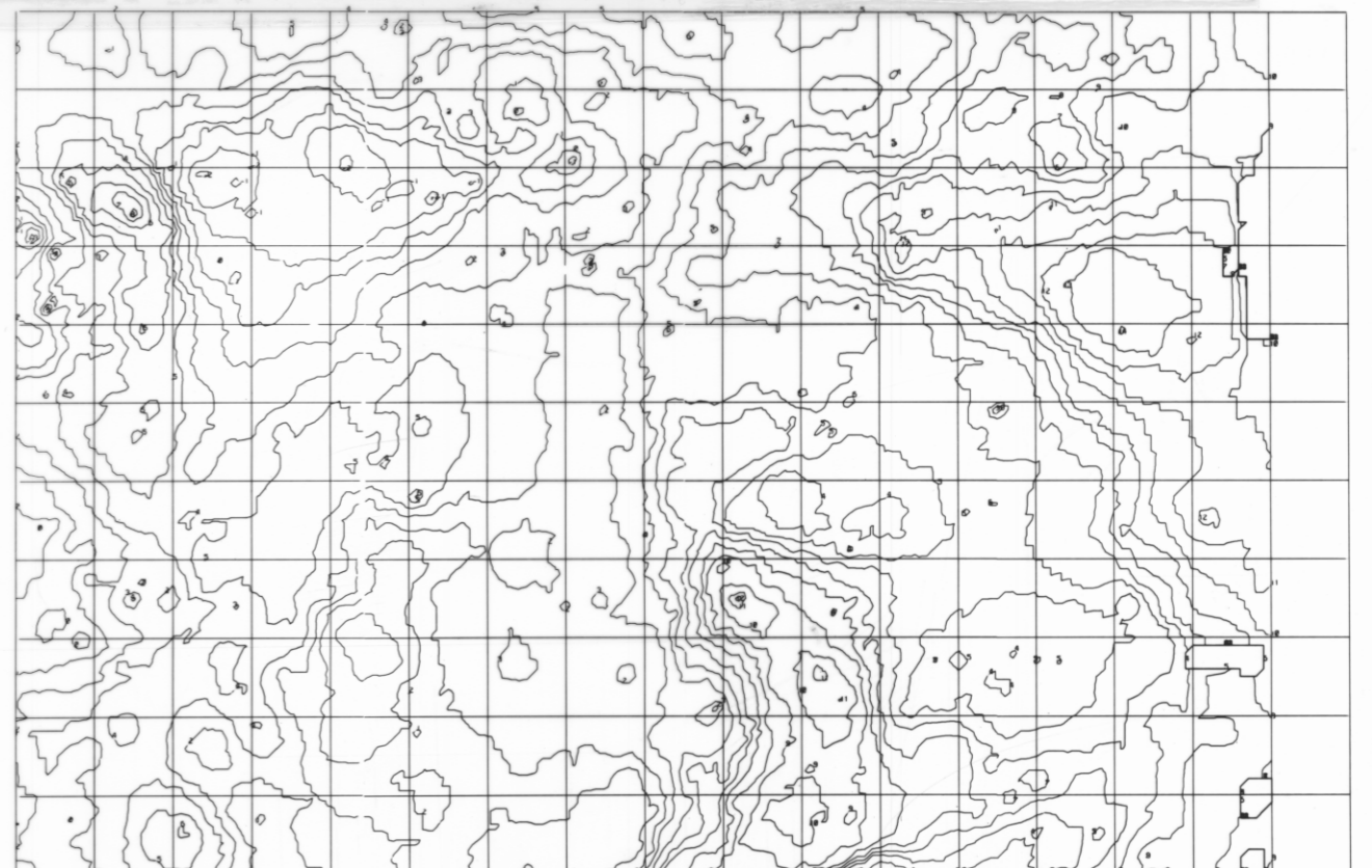
BOUGUER ANOMALIES — DAVIS
