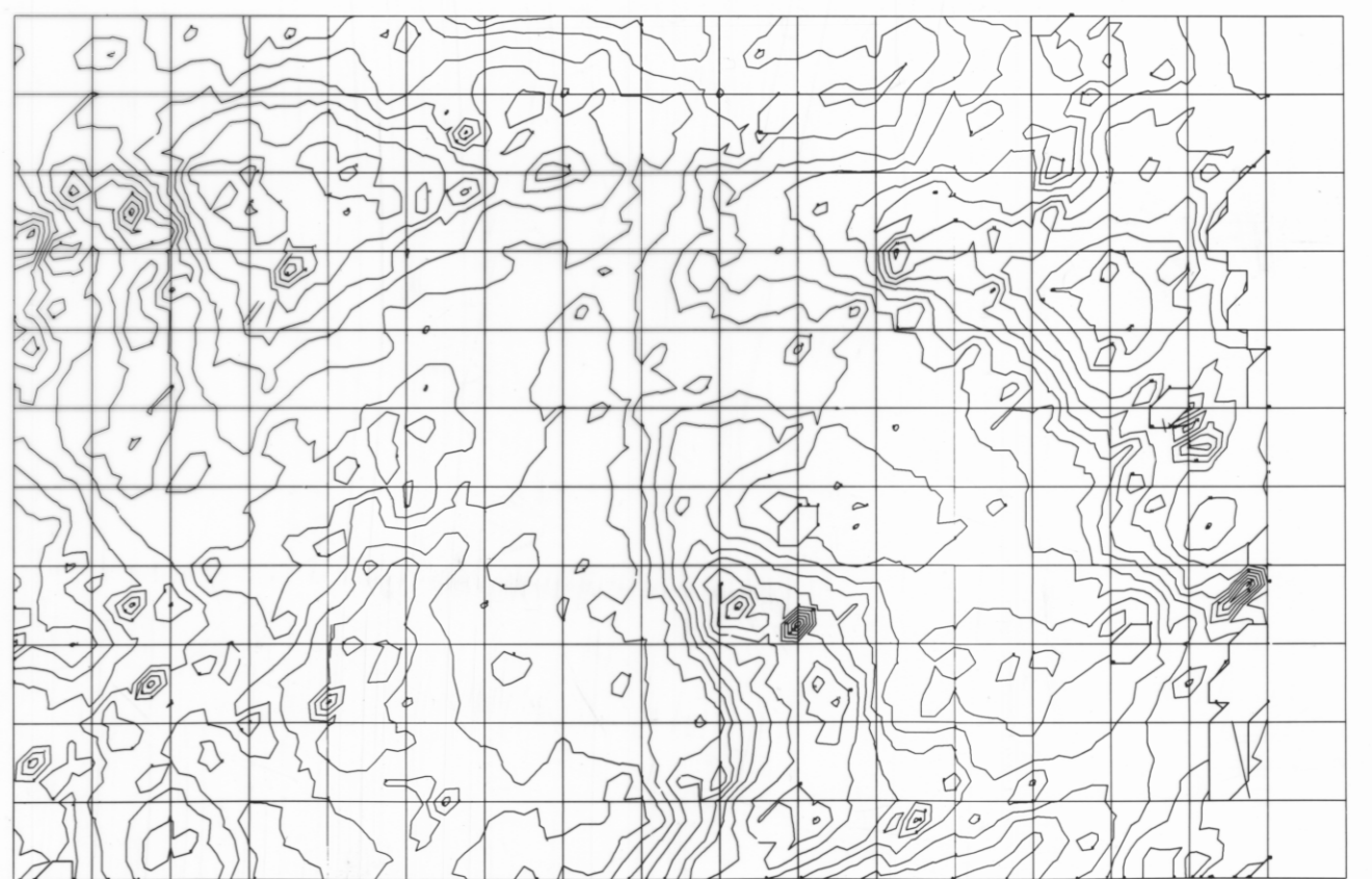
BOUGUER ANOMALIES — KANSAS
