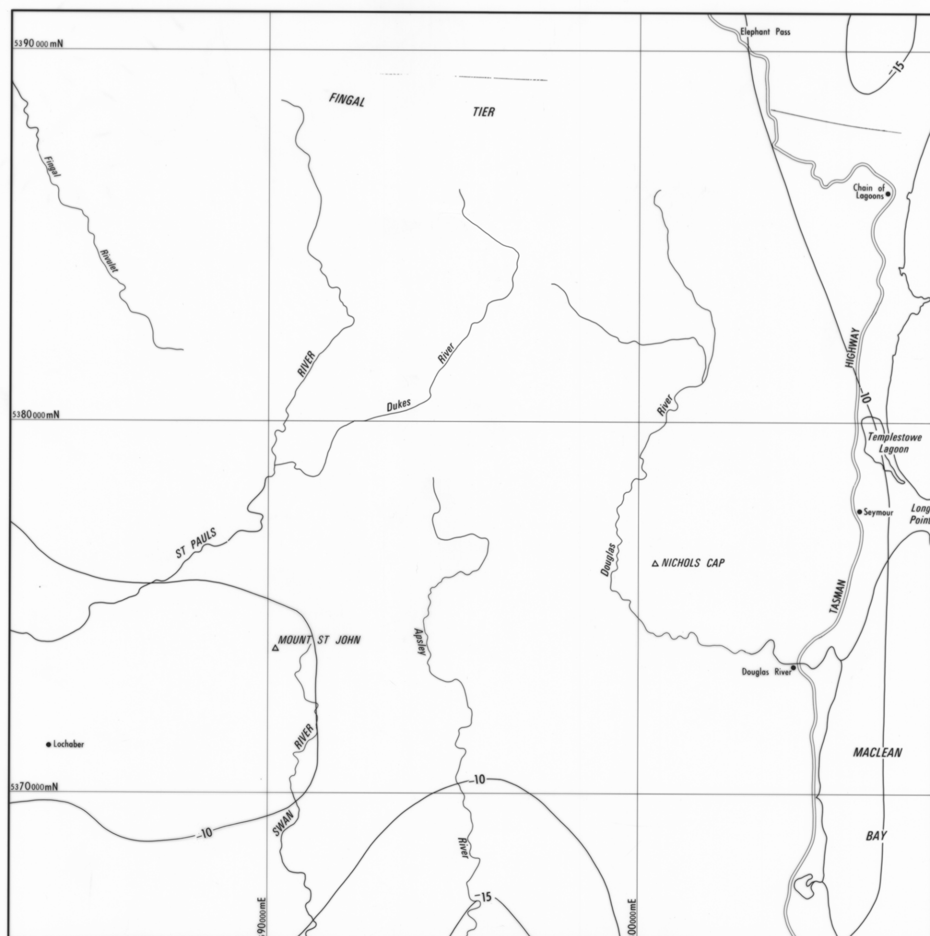
GRANITE
