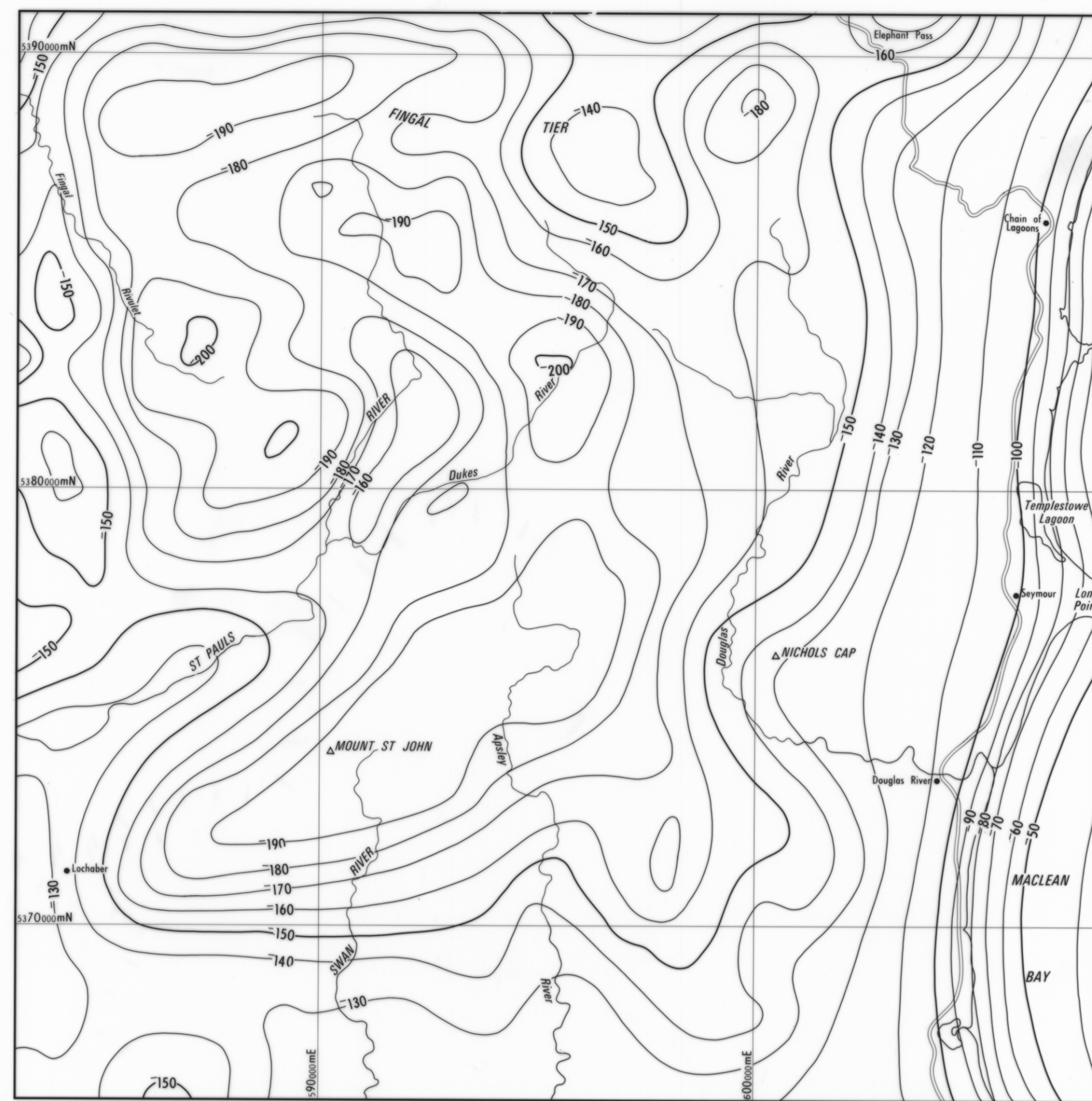
COAL MEASURES
