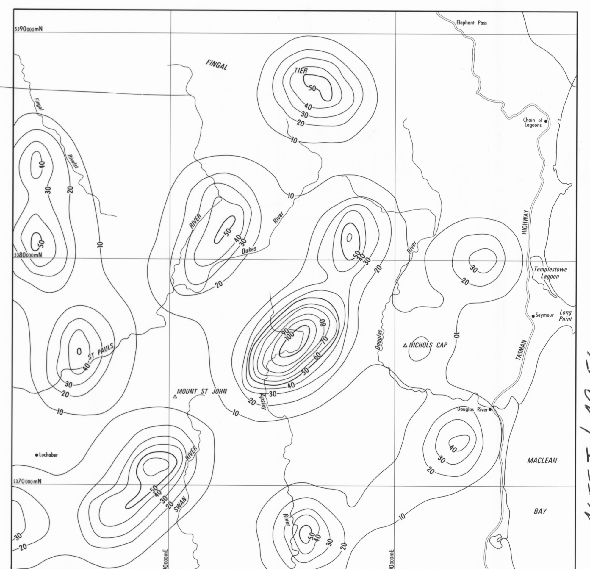
DOLERITE FEEDERS
