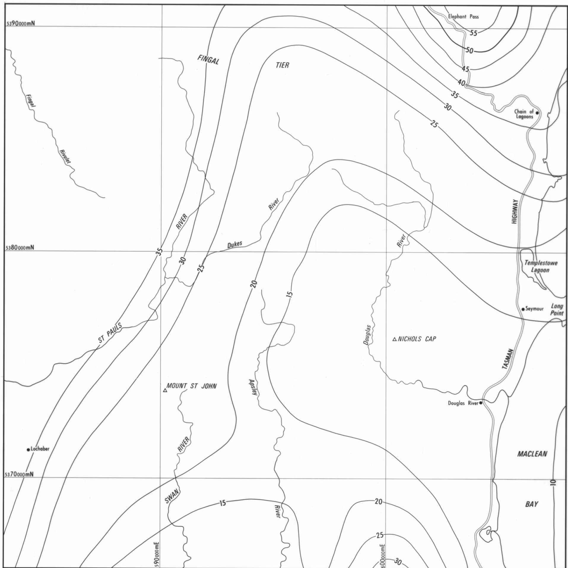
MATHINNA BEDS
