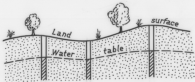
Fig. 6b UNCONFINED WATER
