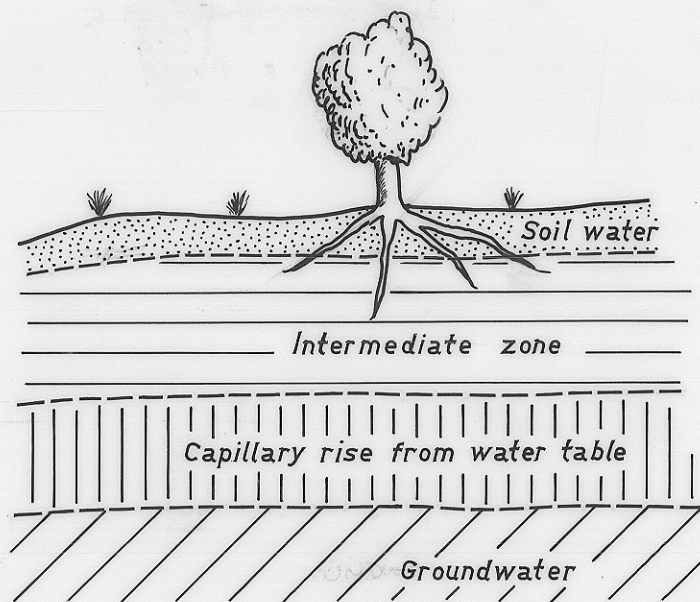
Fig. 6a. GROUNDWATER ZONES
