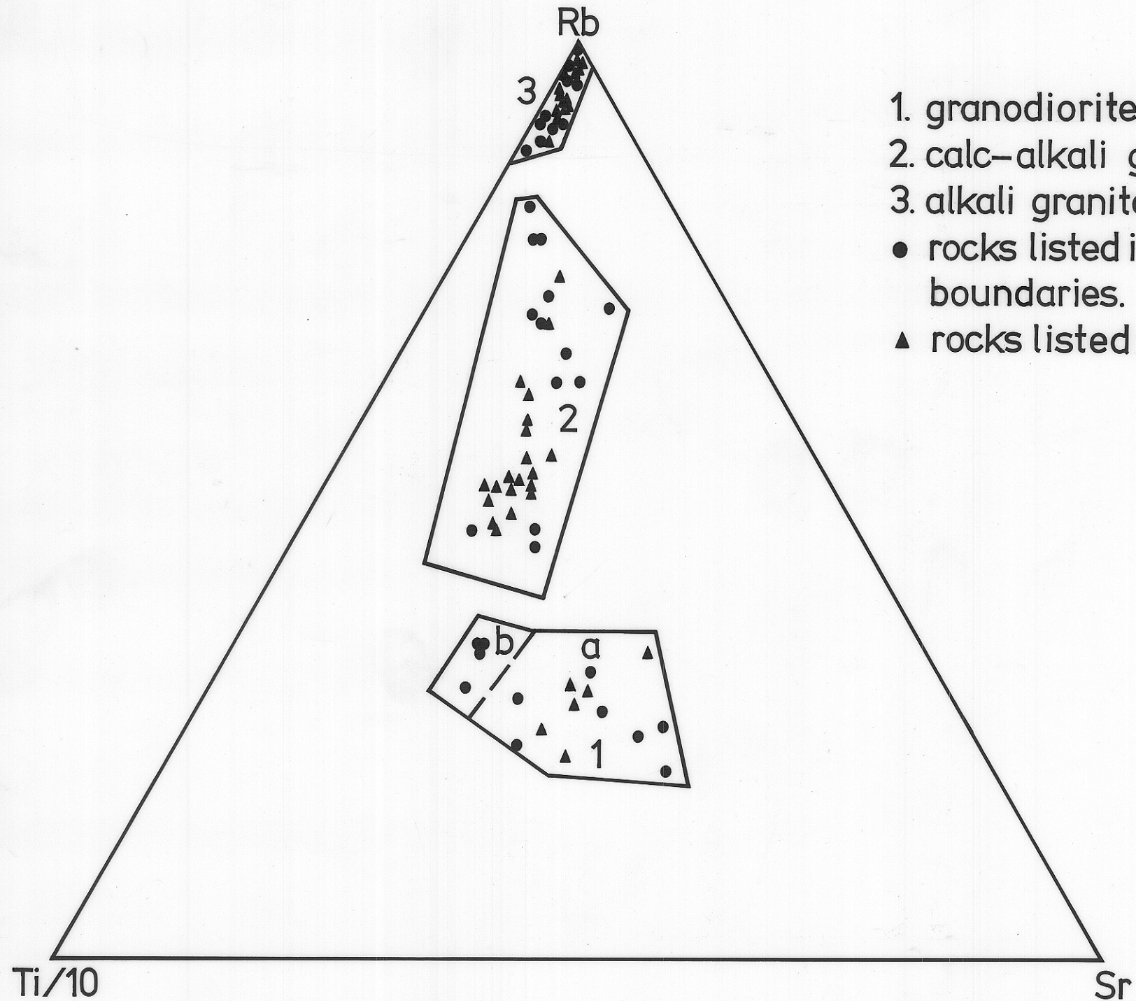
Ti/10 – Rb – Sr DIAGRAM SHOWING ROCKS FROM THE BLUE TIER BATHOLITH LISTED IN GROVES (1977) & IN THIS REPORT.
