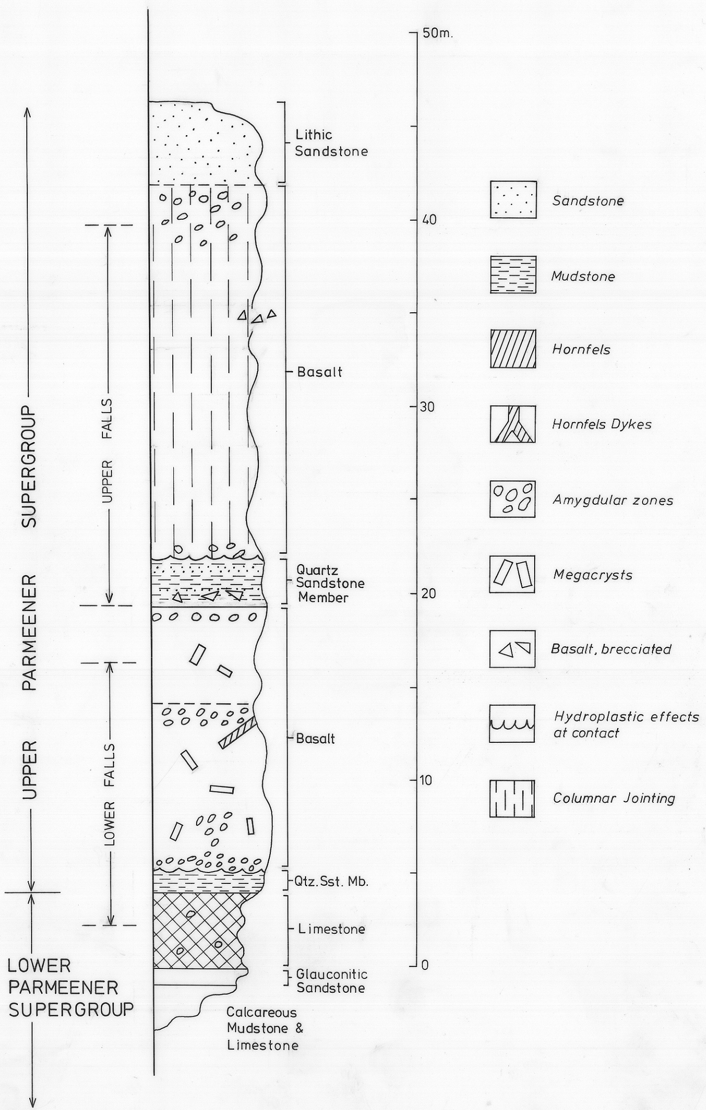
WEBBER FALLS LITHOLOGY
