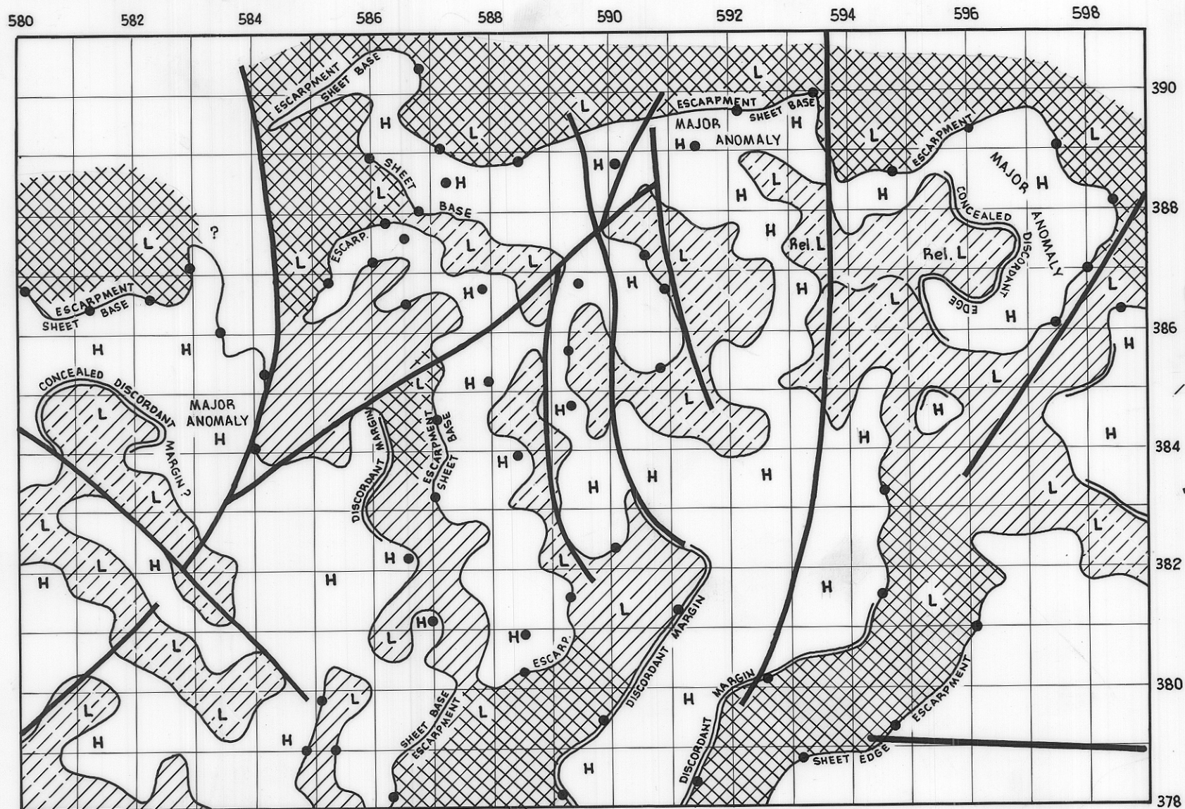
QUALITATIVE INTERPRETATION-FINGAL TIER AEROMAGNETIC SURVEYS
