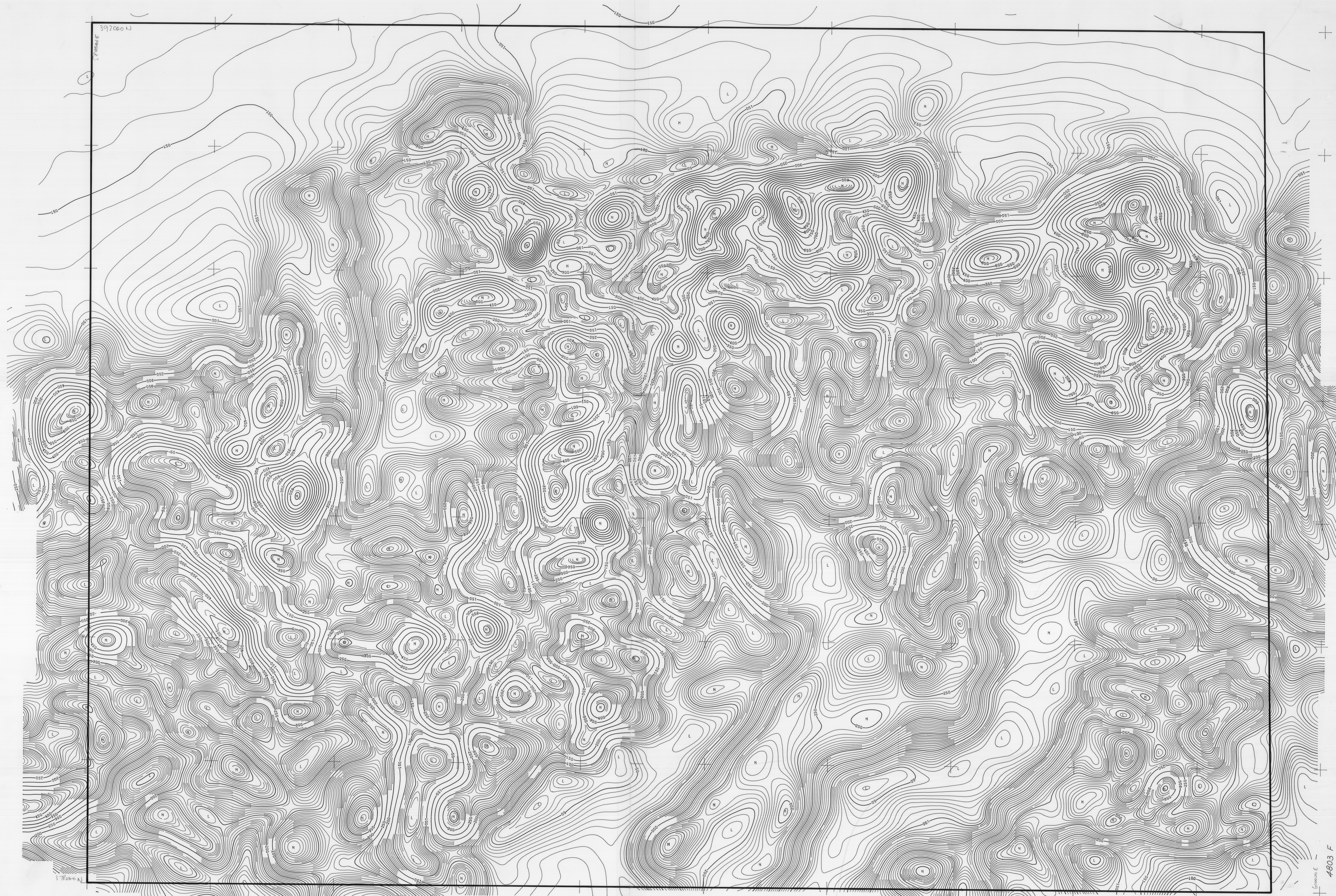
FINGAL TIER AREA AEROMAGNETIC TOTAL INTENSITY CONTOURS LOW ALTITUDE SURVEY CONTOUR INTERVAL 5 nT
