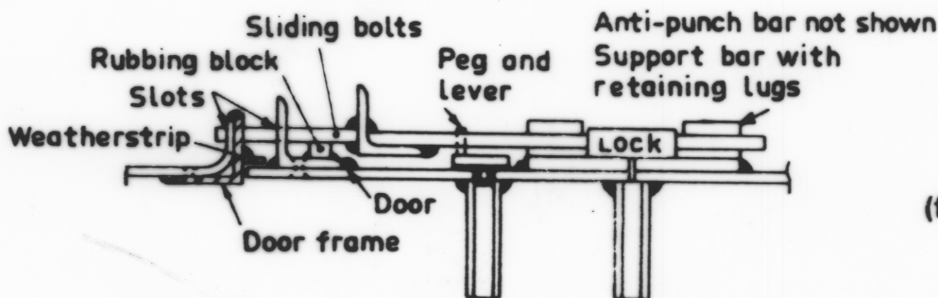
(e) SECTION SHOWING TYPICAL LOCK ARRANGEMENT
