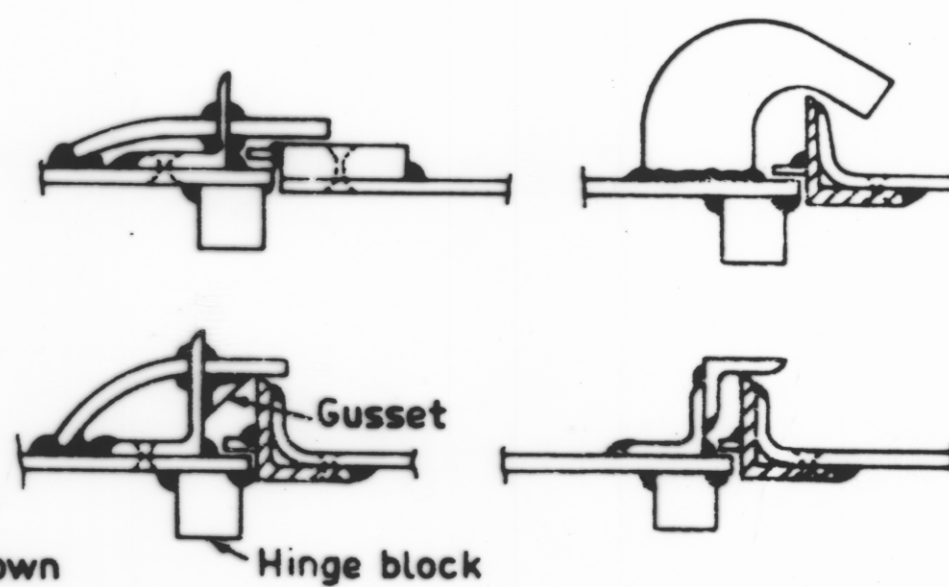
(ii) Four types of door arrangements (hinged side)
