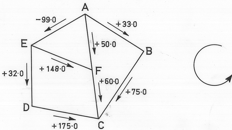
NETWORK ADJUSTMENT
