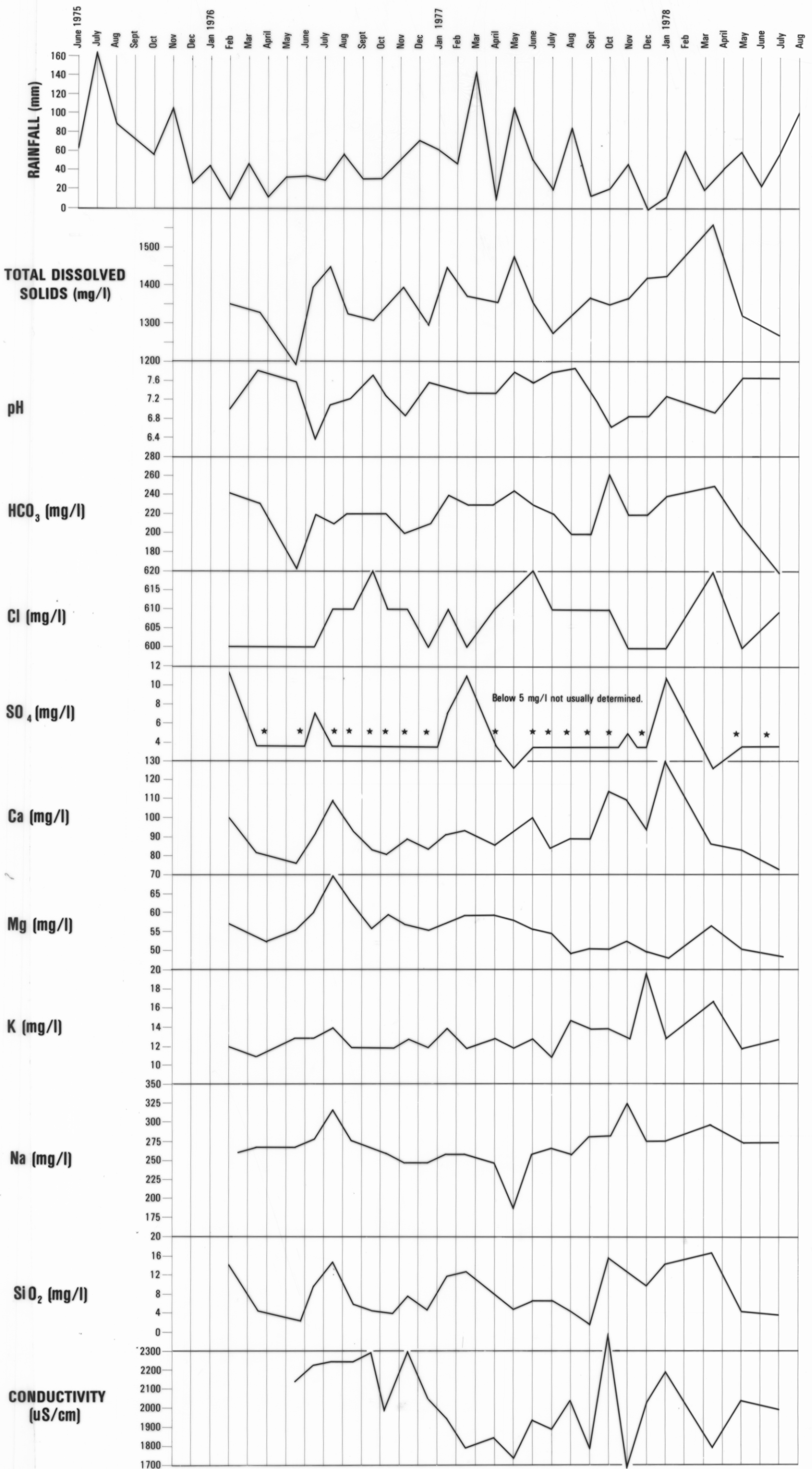
VARIATION OF WATER QUALITY WITH TIME, IH 3 (CRESSY)
