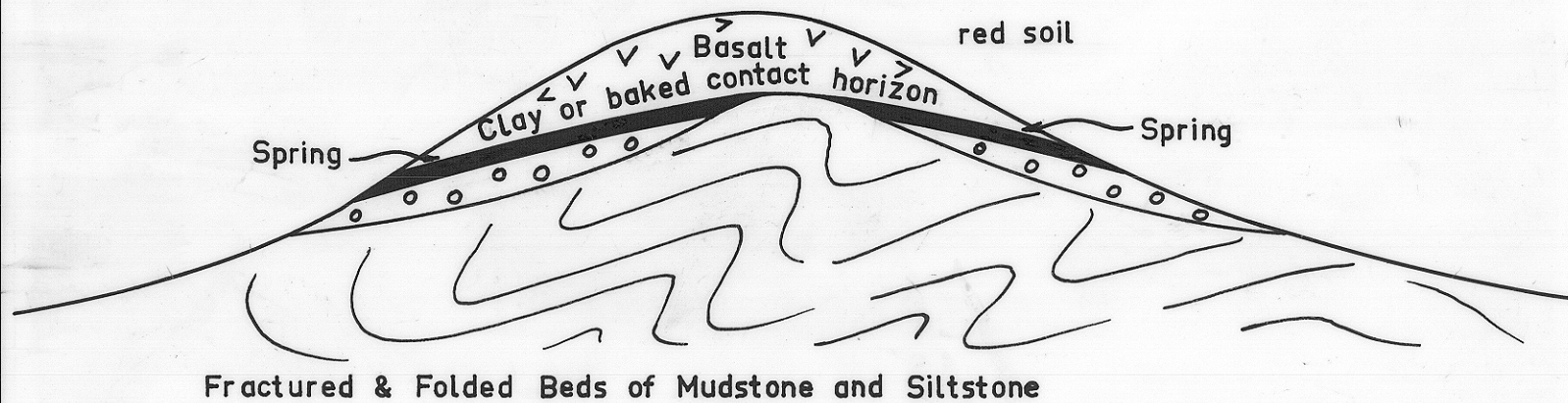
Basalt Lava flow over a former ridge
