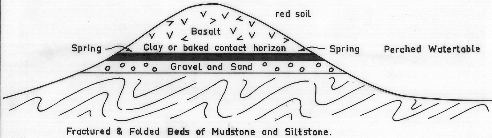
Basalt Lava flows over a surface of little relief
