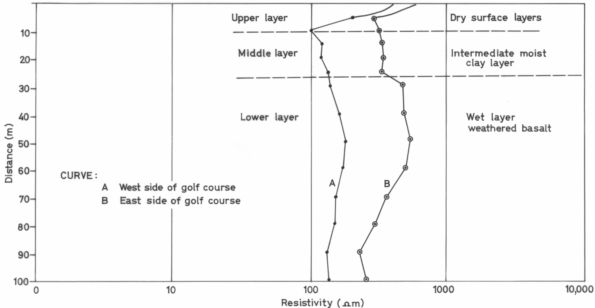
Fig.2 RESISTIVITY PROBE SCOTTSDALE GOLF COURSE (Wenner Configuration)
