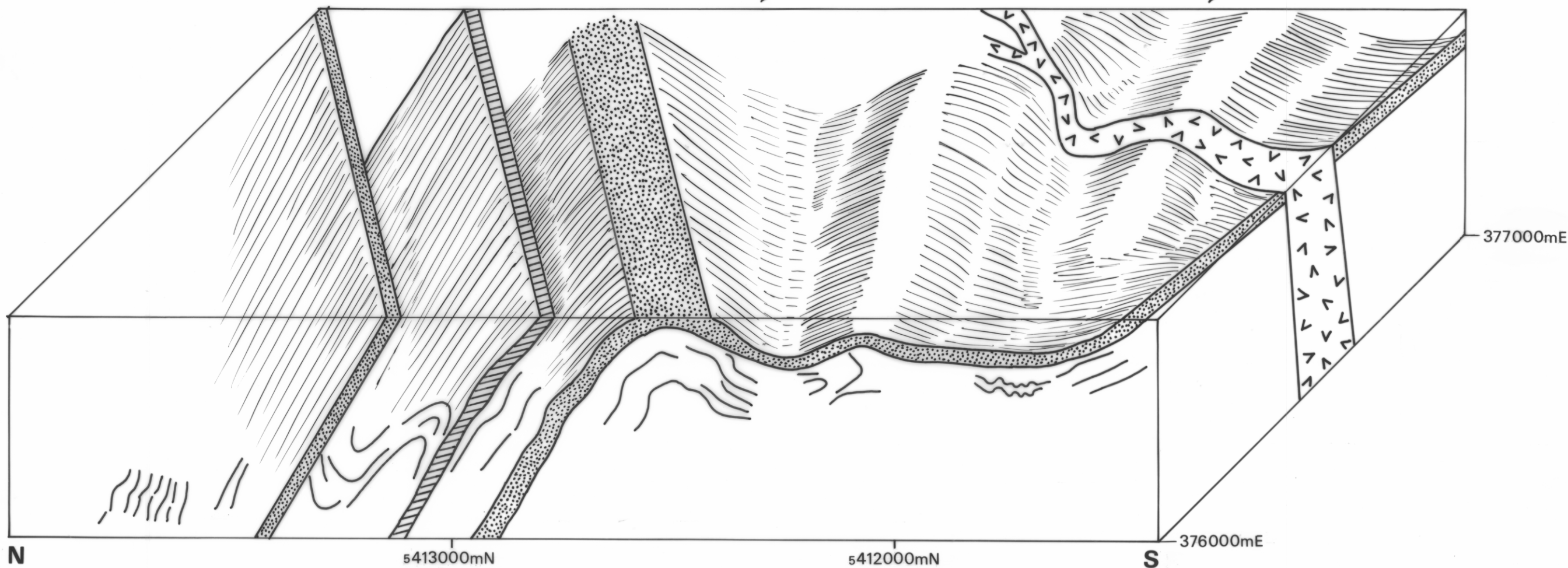
BLOCK DIAGRAM D3 STRUCTURE — MT. BISCHOFF
