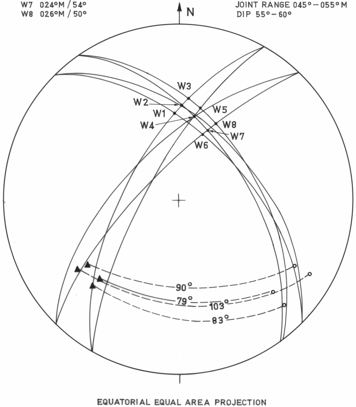
ANALYSED POTENTIAL WEDGE FAILURE BASS HIGHWAY CUTTING
