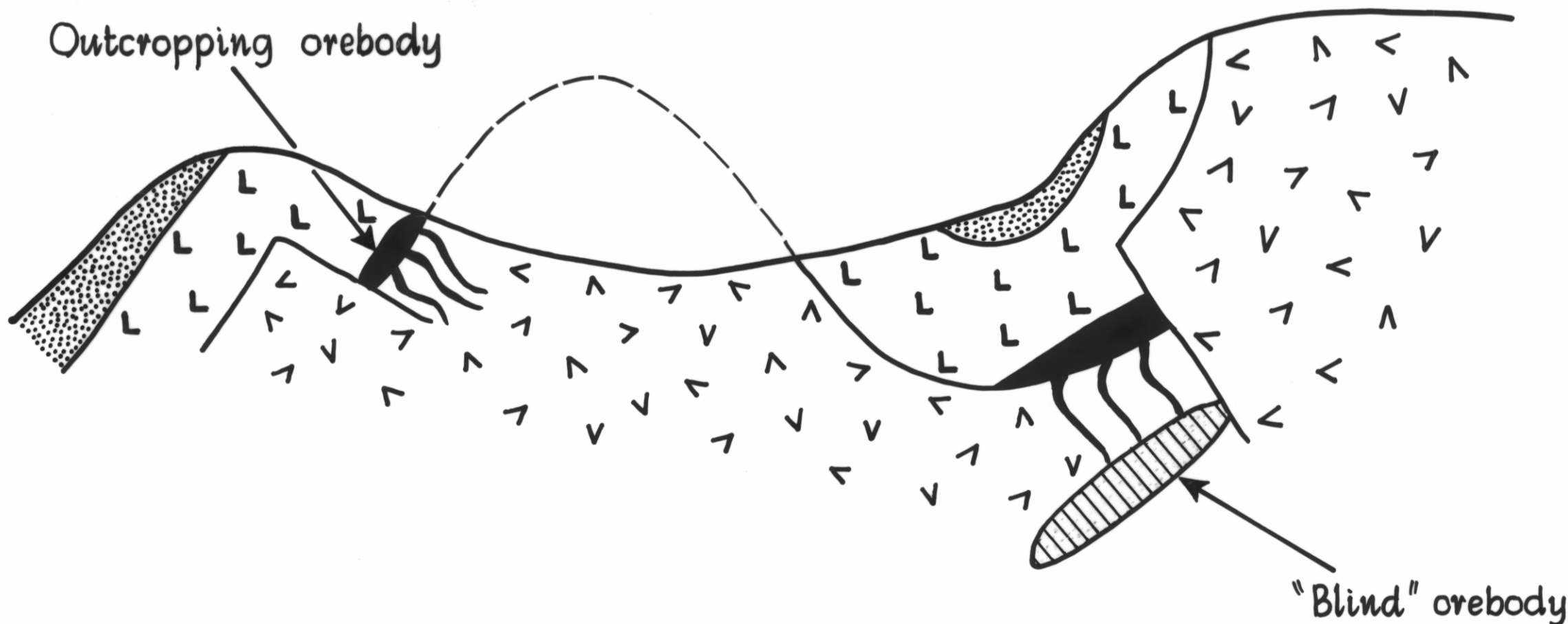
(c) CONFIGURATION OF OREBODIES AFTER FOLDING & EROSION
