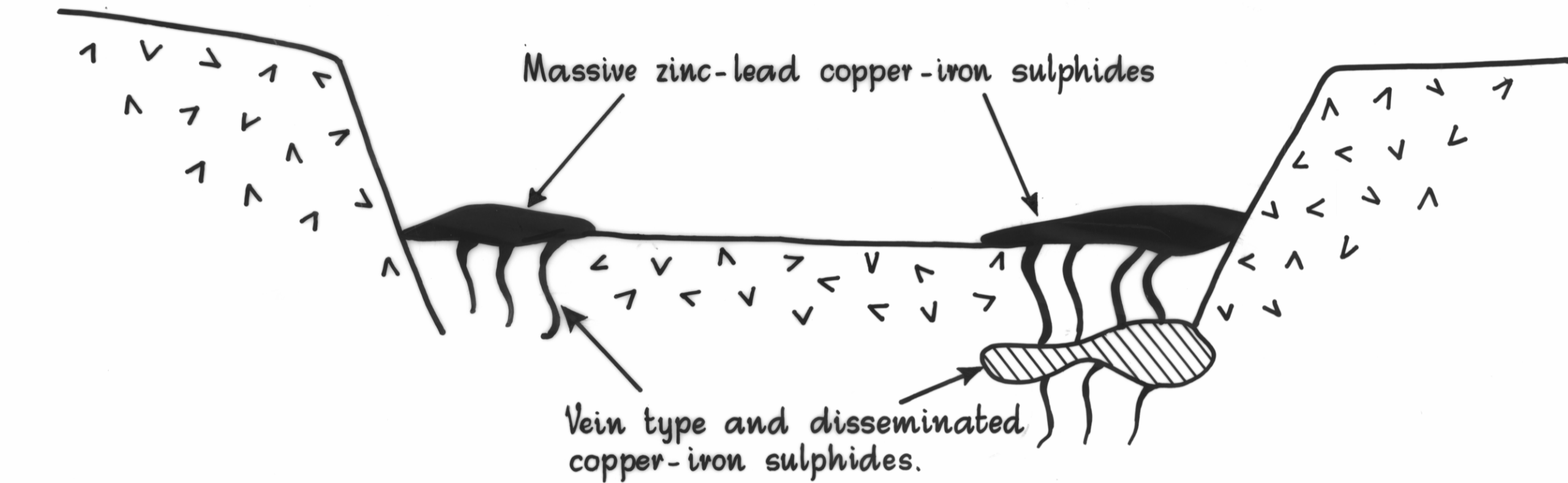
(a) FORMATION OF ORES AT OR NEAR SEA FLOOR DURING PAUSE IN VOLCANISM
