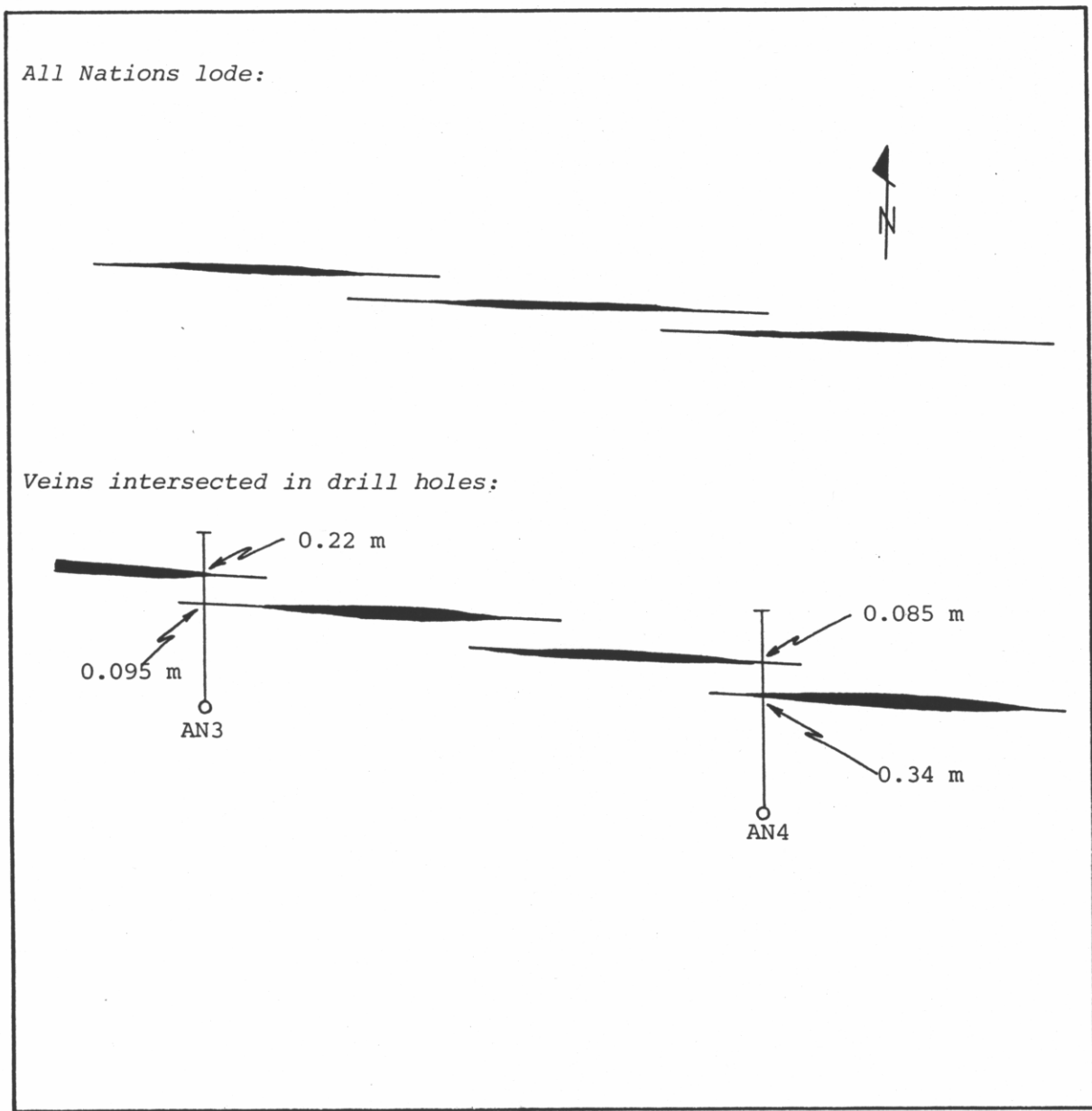
Figure 10. Sketch plan showing possible drill hole intersections in an echelon vein system, All Nations mine.
