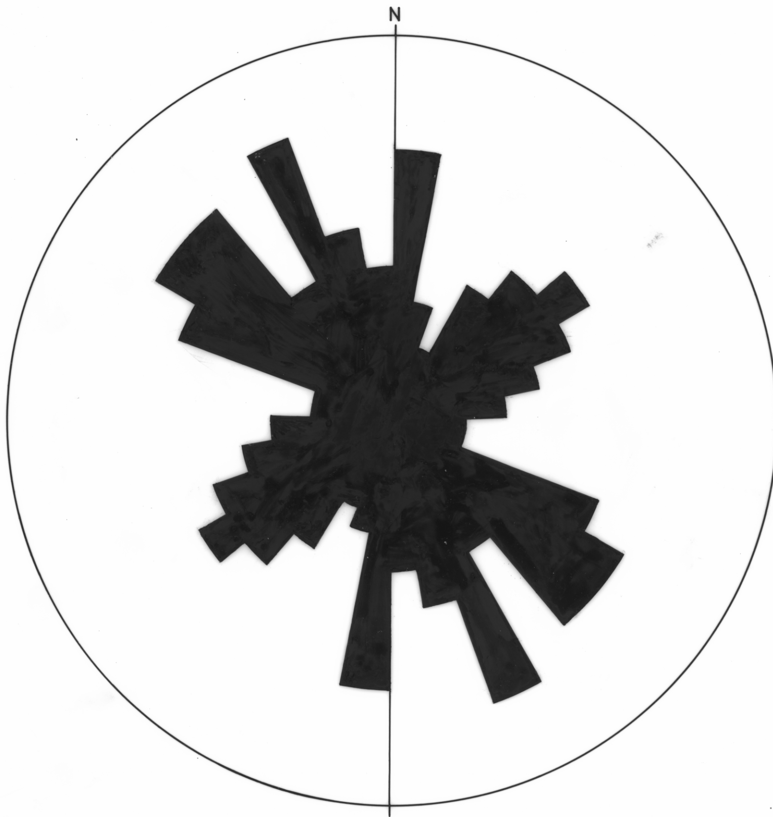
Distribution of faults on the Sorell sheet
