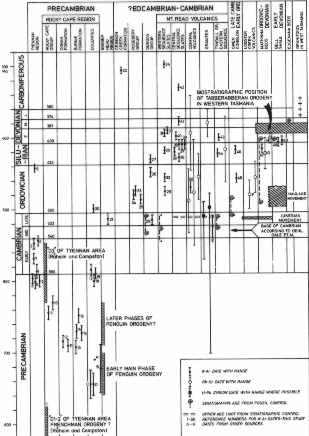
Fig.6. Radiometric ages plotted according to stratigraphic units
