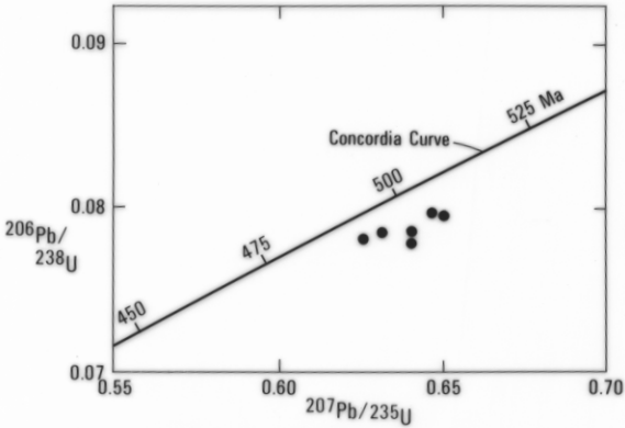
a Quartz Porphyry in Western Sequence.
