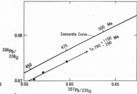
b Pumphouse Porphyry
