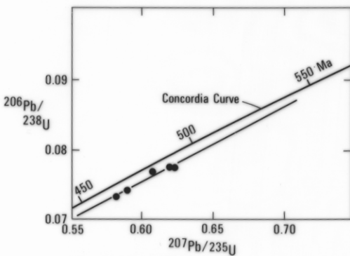
e Tyndall Group Tuff
