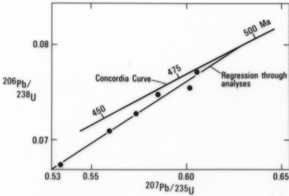
c Murchison Granite
