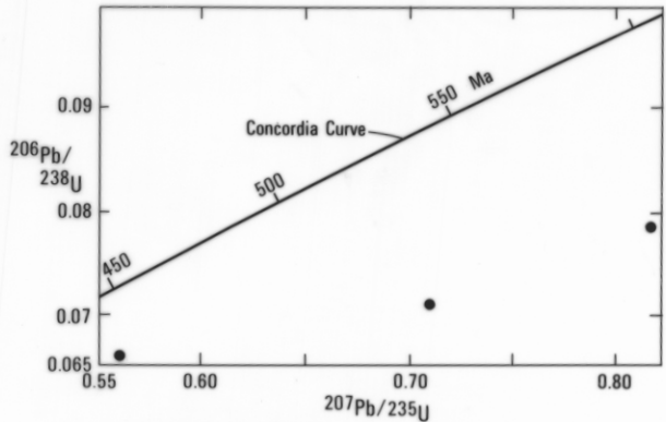
f Lobster Creek Volcanics
