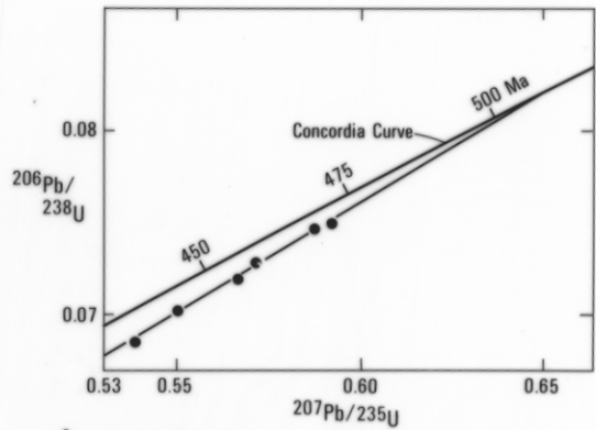
d Darwin Granite
