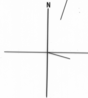
Crossbedding
