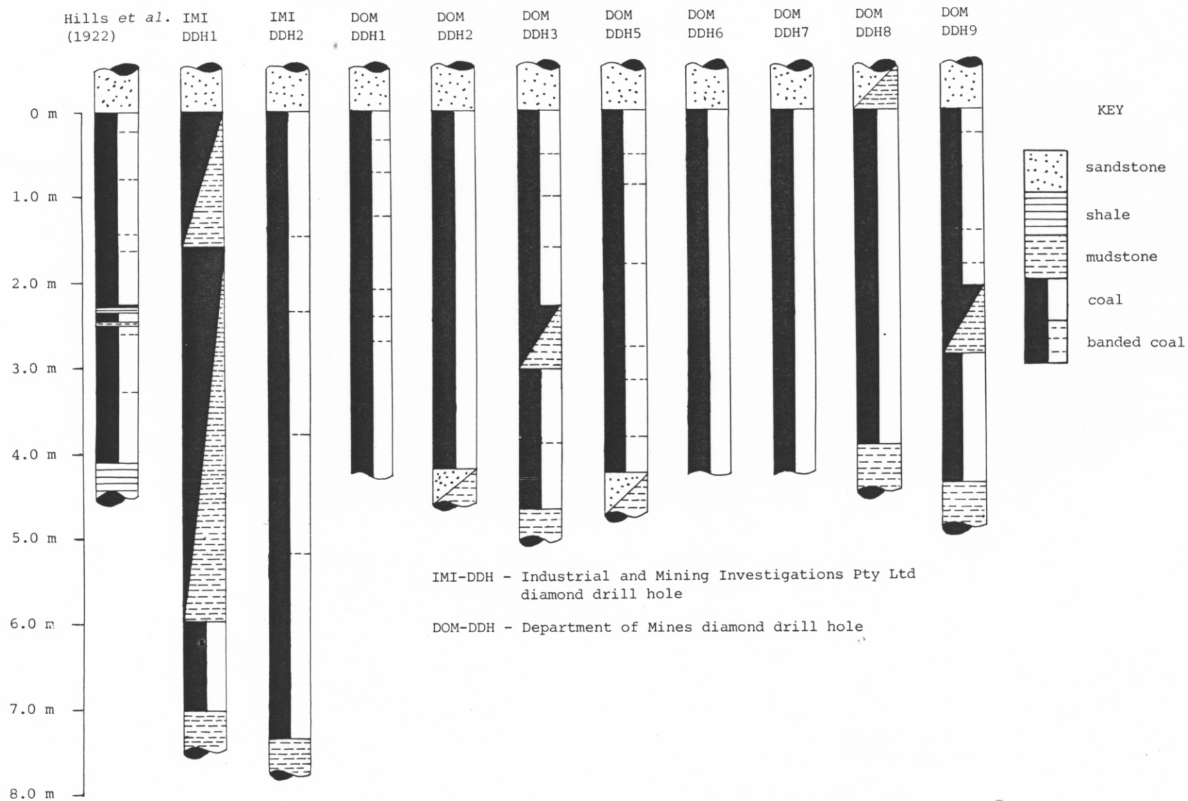
Figure 2. Seam sections of the DB (mined) seam, Dalmayne.
