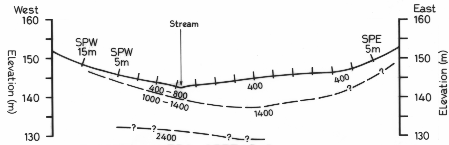
VELOCITY LAYERS, SPREAD 5
