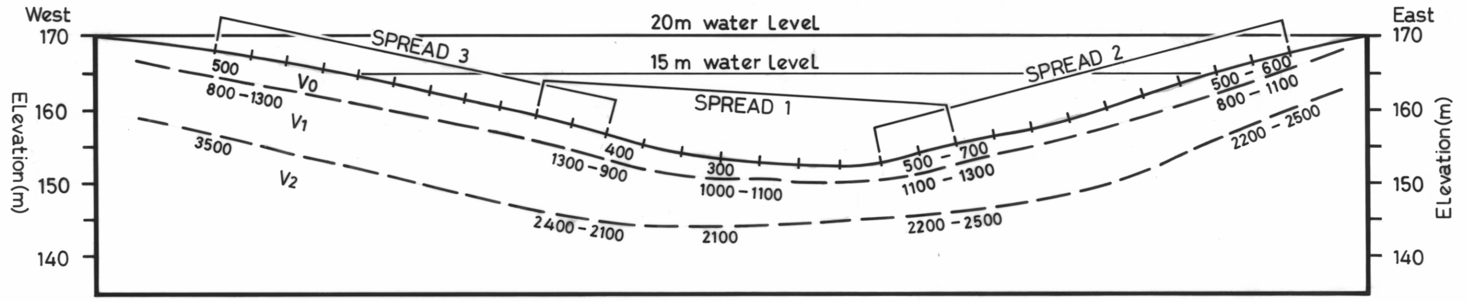
VELOCITY LAYERS ACROSS PROPOSED CENTRELINE
