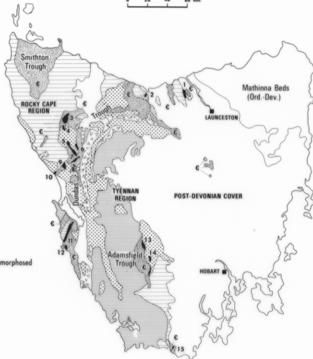
Schematic geological map of Tasmania showing location of ultramafic-mafic complexes
