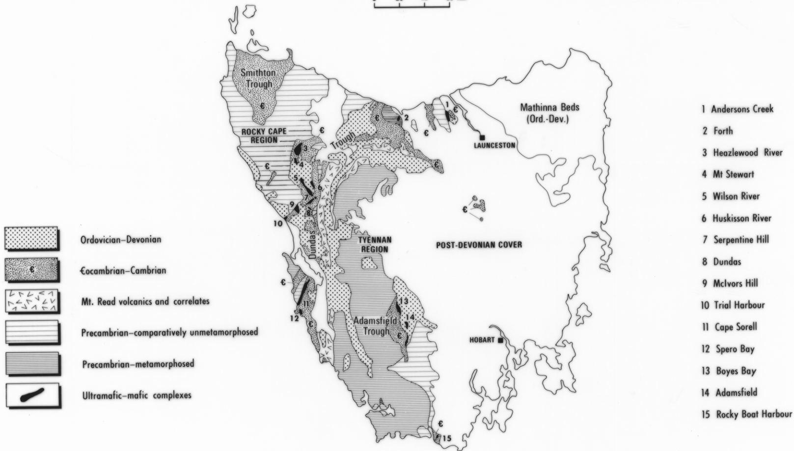
Schematic geological map of Tasmania showing location of ultramafic–mafic complexes
