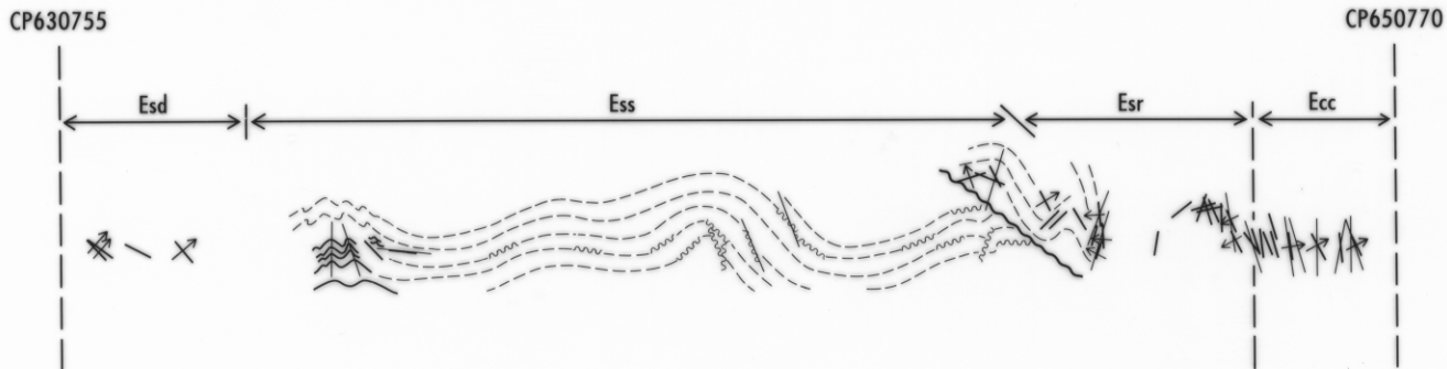
Figure 9. Structural cross-section — projection plane 055^{\circ}/90 between CP630755 and CP650770. Produced from data enclosed by parallelogram CP630755, CP650770, CP657755, CP637740.
