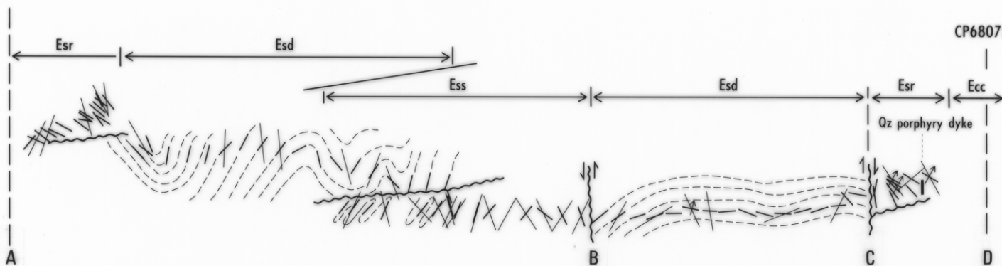
Figure 11. Interpretative structural section — projection plane V/055 between CP657713 and CP680728. Produced from data enclosed by CP657713, CP680728, CP690710, CP670696, but only partially presented on Figure 1.
