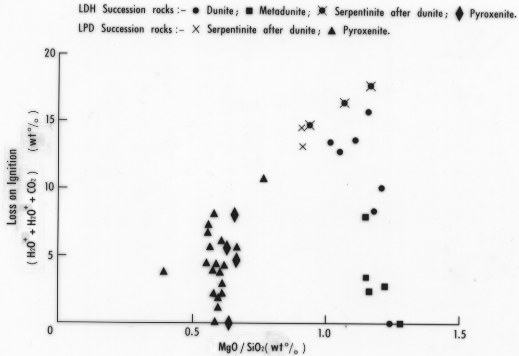
Fig.47 Loss on Ignition ~ MgO/SiO 2 (wt%). Degree of isochemical serpentinisation. Samples on base line represent parental compositions based on mineral chemistry.
