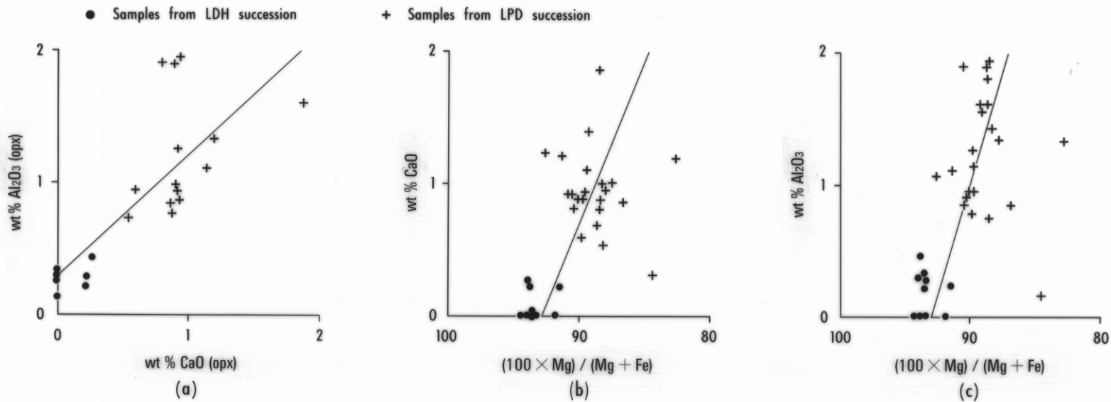
Fig. 49 Chemical variation diagrams for orthopyroxene — (a) \text{Al}_2\text{O}_3 \sim \text{CaO} , (b) \text{CaO} \sim \text{Mg}^* , (c) \text{Al}_2\text{O}_3 \sim \text{Mg}^* .
