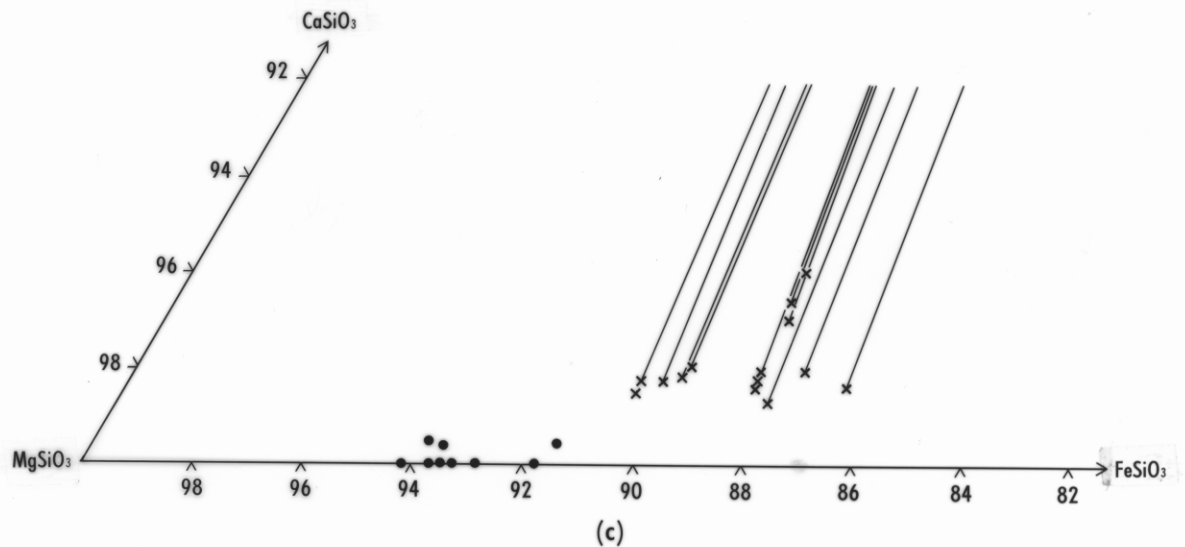
Fig. 50 (a) Part of the pyroxene quadrilateral, showing area of plot of orthopyroxene from the LDH succession (fig (c)), and orthopyroxene + coexisting clinopyroxene (hatched areas with boundary tie lines) from the LPD succession (figs (b), (c)). (b) Part of the pyroxene quadrilateral, showing compositions and direction of tie lines for clinopyroxene from the LPD succession (compositions tables 15 and 23). (c) Part of the pyroxene quadrilateral, showing compositions and direction of tie lines for orthopyroxene from the LPD succession (crosses), and composition of orthopyroxene from the LDH succession (dots), (compositions tables 17 and 22).
