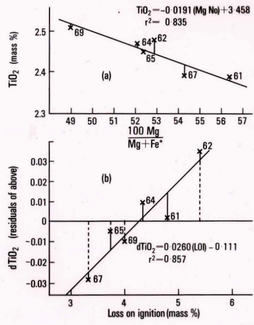
Figure T(a) Webber Falls Basalt - upper unit - TiO_2 versus Mg number. Figure T(b) Webber Falls Basalt - apparent increase in TiO_2 content with alteration.
