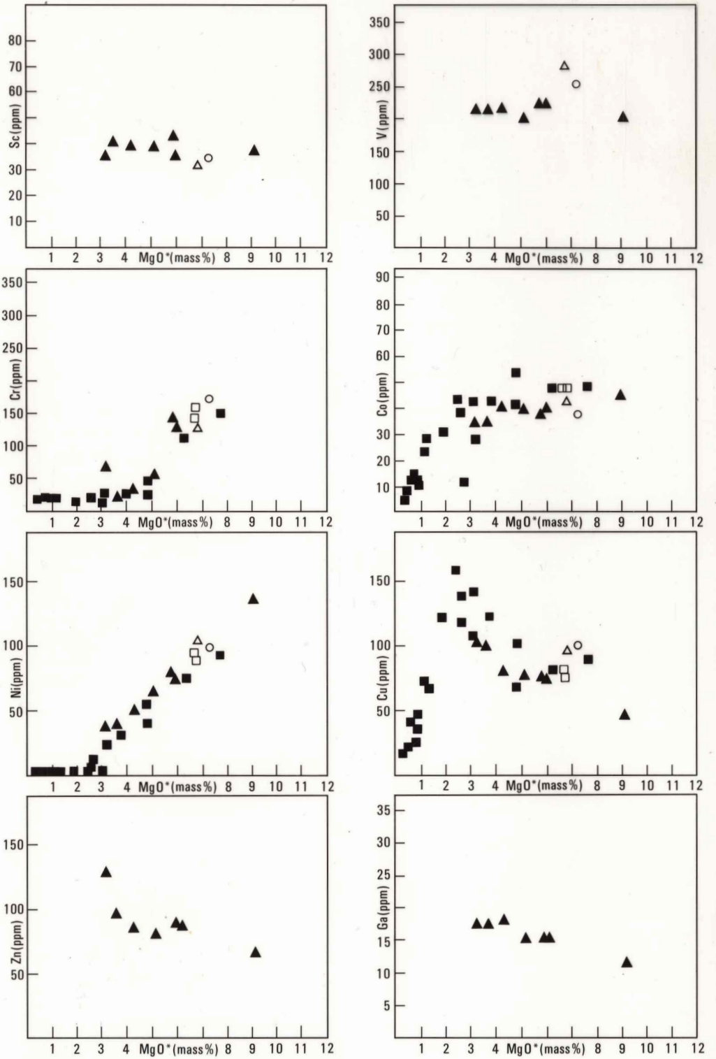
FIGURE D3(a) Fingal Tier and elsewhere in Tasmania, differentiation of dolerite.
