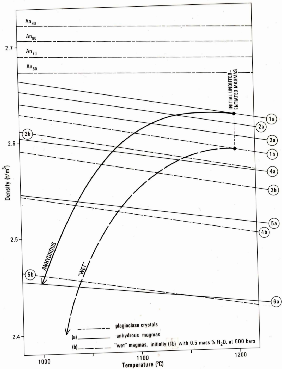
FIGURE D5. Density of plagioclase crystals and undifferentiated doleritic magma
