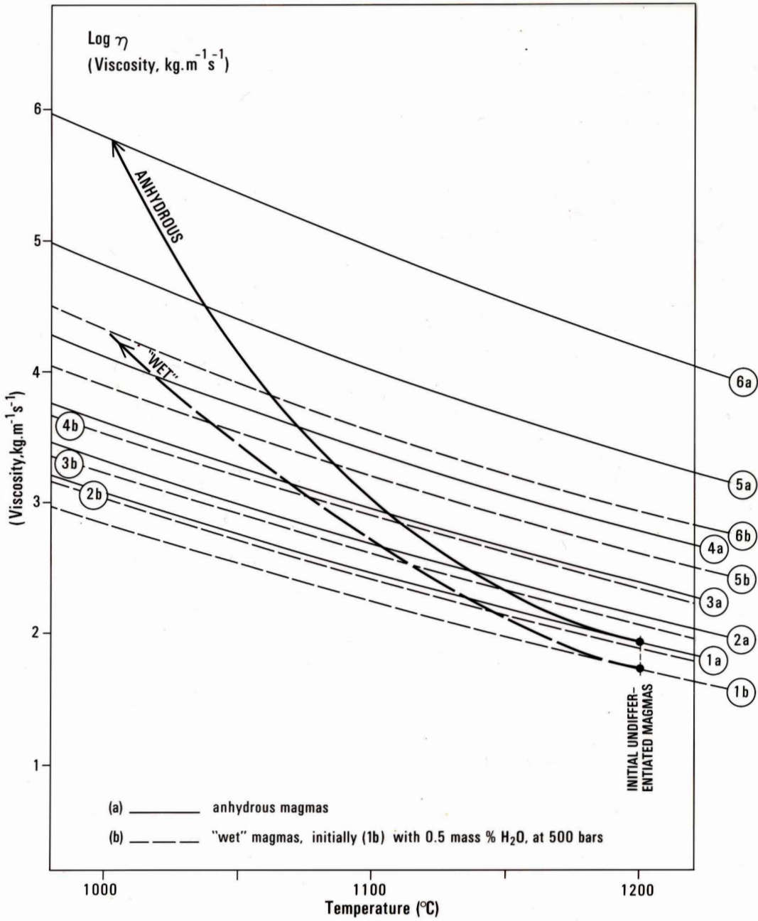
FIGURE D6. Viscosity of undifferentiated doleritic magma
