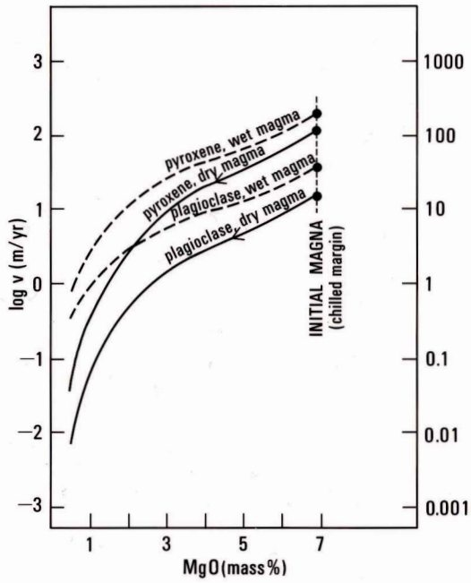
FIGURE D7. Stokes-Law settling velocities of pyroxene and plagioclase crystals.
