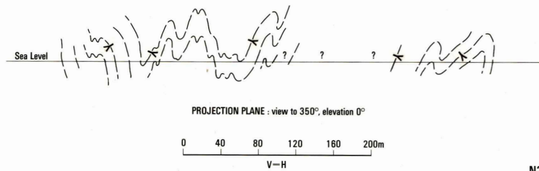
PICCANINNY POINT-FOLD PROFILE
