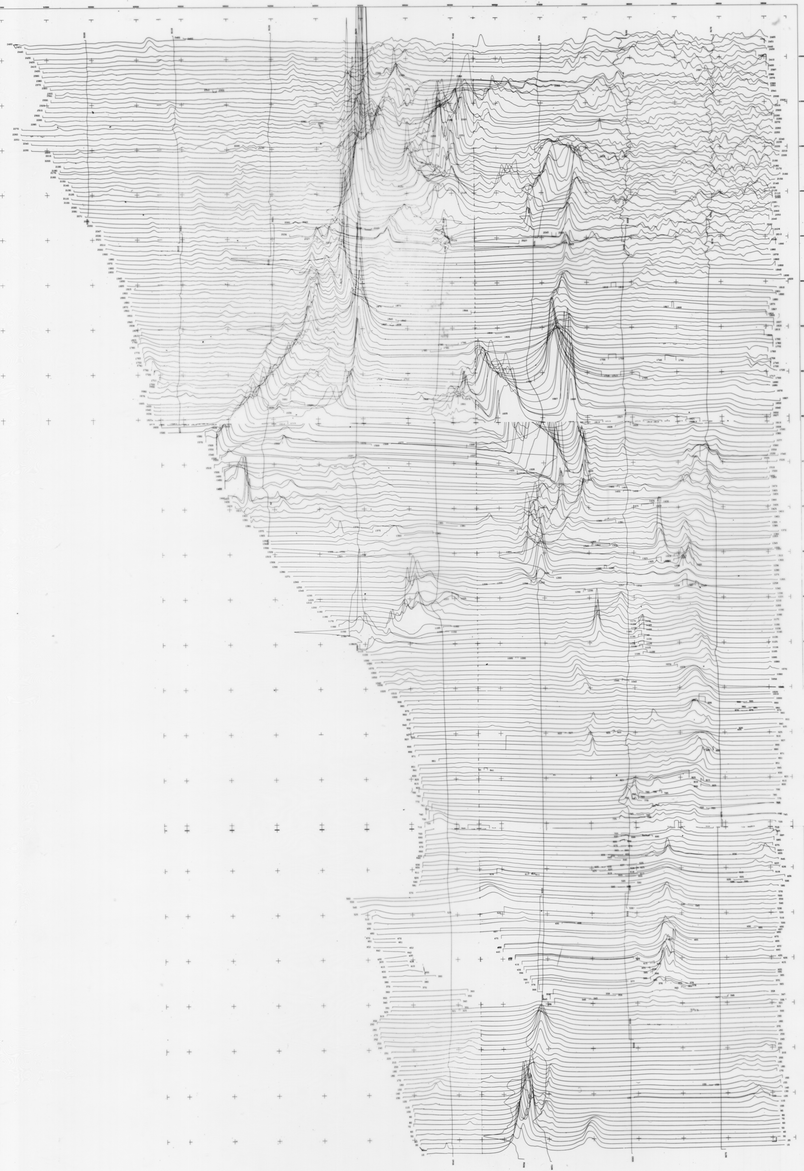
FIGURE 3-2 STACKED PROFILES WEST TASMANIA (1981) AEROMAGNETIC SURVEY
