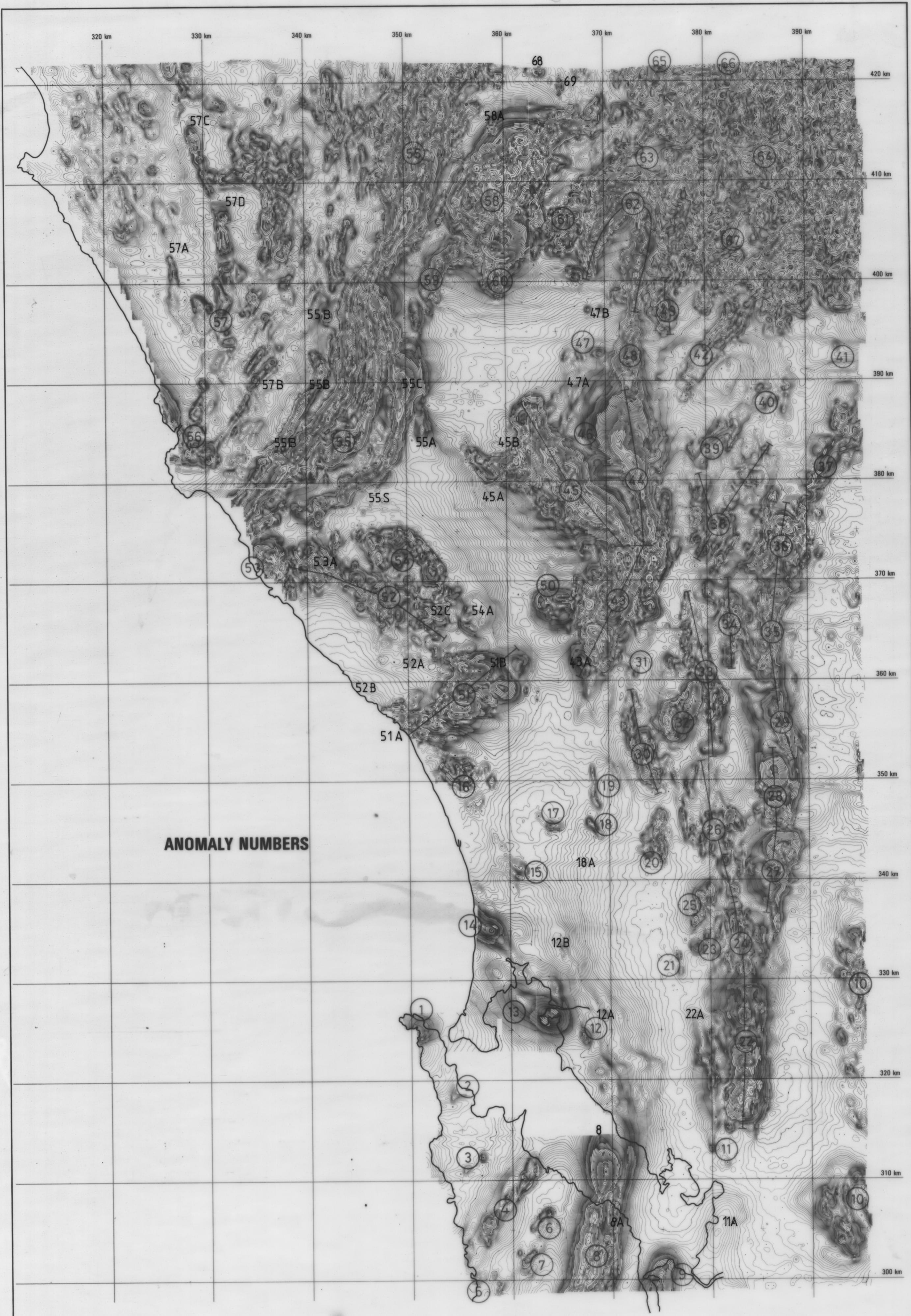
FIGURE 3-3 MAGNETIC FIELD & ANOMALY NUMBERS
