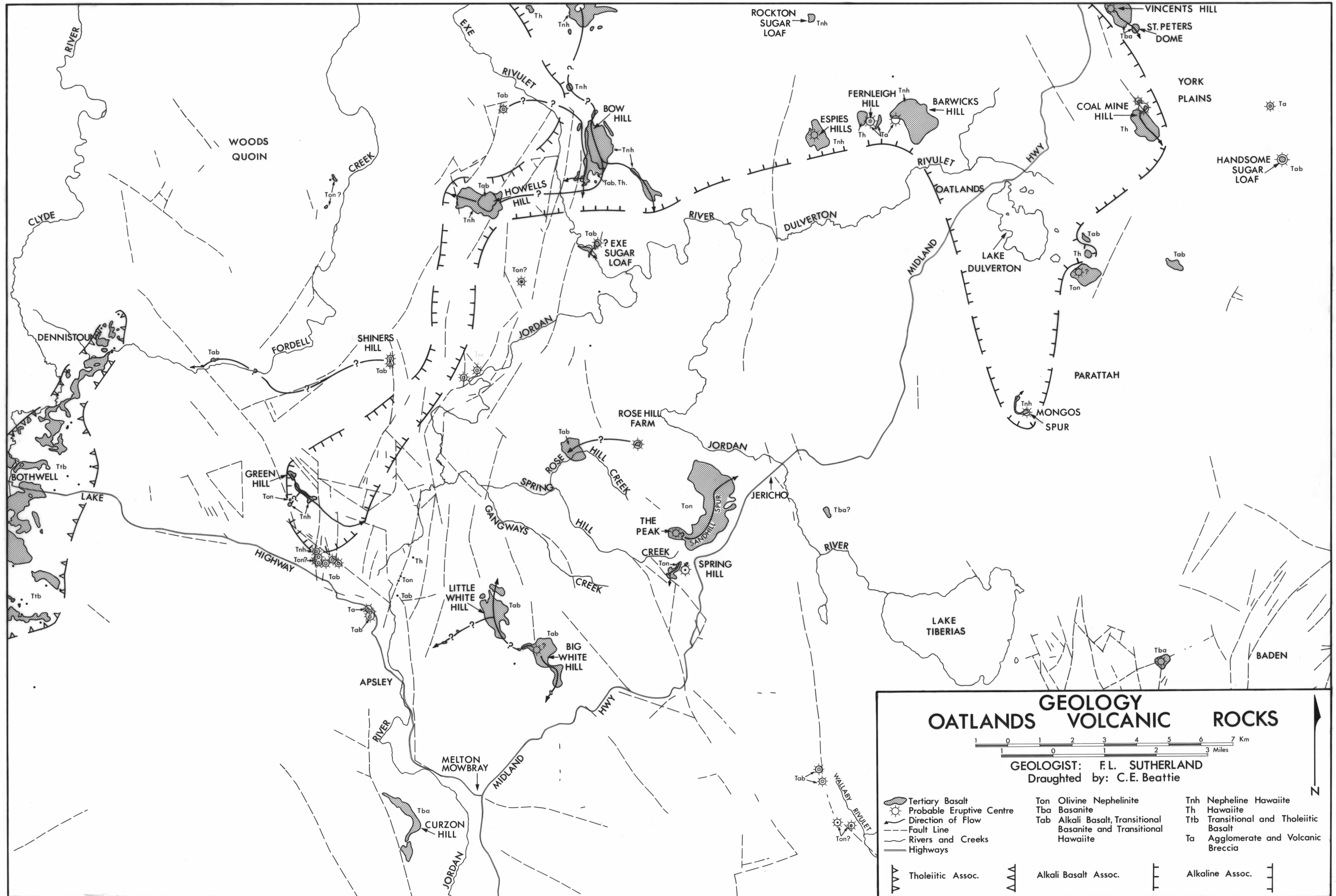
FIGURE 1 Oatlands Volcanic Rocks chapter - Sutherland.
