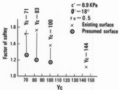
FACTOR OF SAFETY Vs. SURFACE SHAPE (c)
