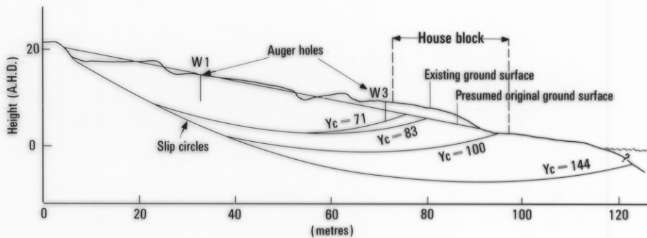
FAILURE PLANE LOCATIONS (a)
