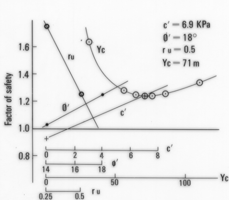
FACTOR OF SAFETY Vs. VARIABLES (b)
