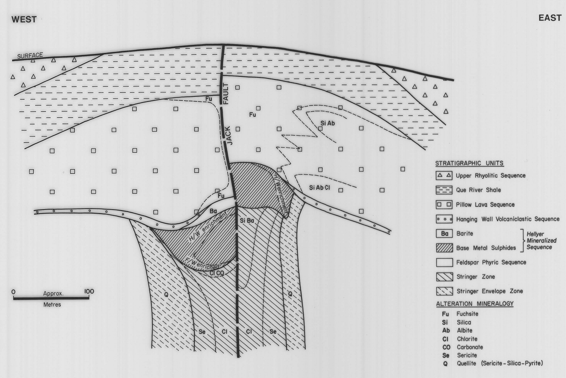
FIG. 2 HELLYER SCHEMATIC CROSS SECTION
